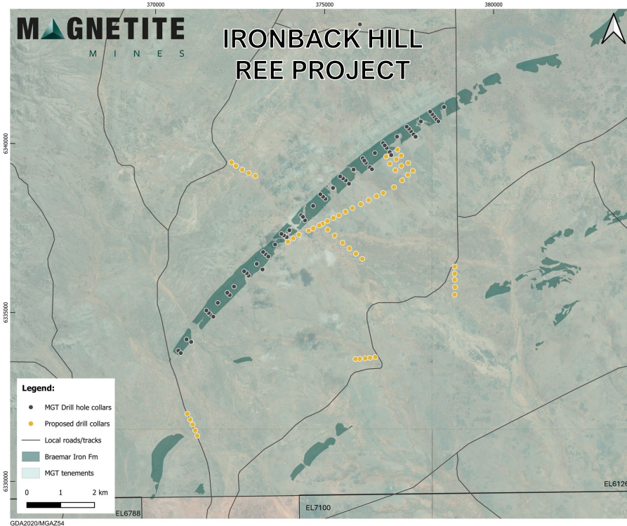
Existing iron ore and planned REE drill hole locations
