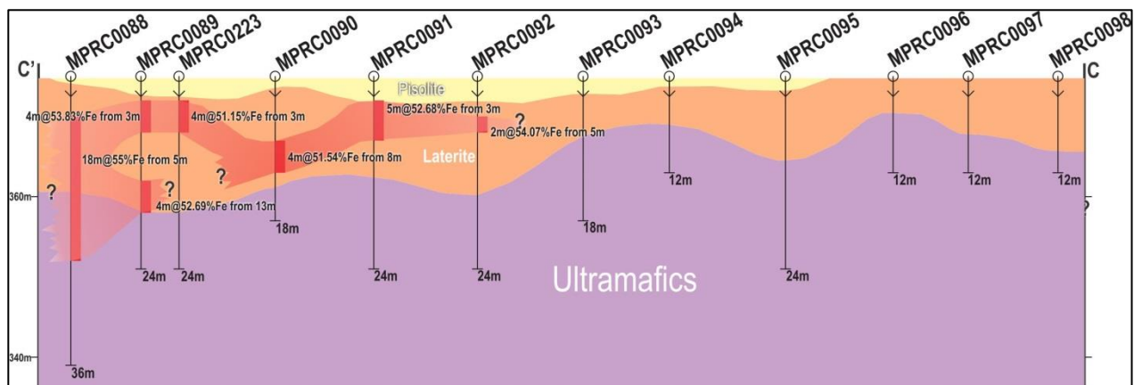
Figure 7: Cross Section C'-C showing the regolith profile for Area 3 and the most significant iron mineralisation intercepts. Cross section shown with 2-times vertical exaggeration.
