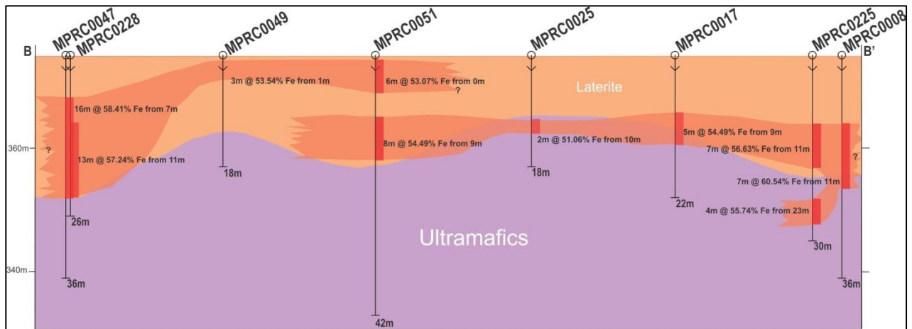
Figure 5b: Cross Section B-B' oriented across the drilling lines showing the regolith profile and the iron mineralisation throughout the drill holes. Cross section shown with 2-times vertical exaggeration.
