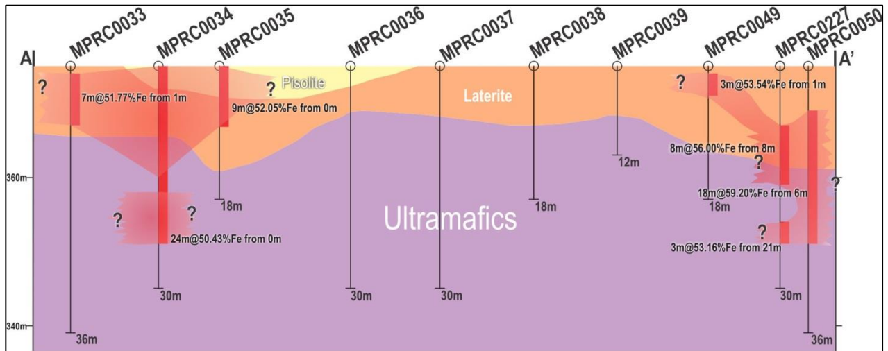
Figure 5a: Cross Section A-A' showing the general regolith profile for Area 2 and the significant iron intercepts. Cross section shown with 2-times vertical exaggeration.
