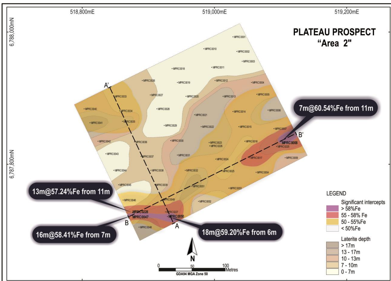
Figure 4: Plan of Area 2 showing the location of the drill holes, the distribution of the laterite depth and contour colours for iron grades. The black dashed lines show the location of the cross sections shown in Figures 5a and 5b below.
