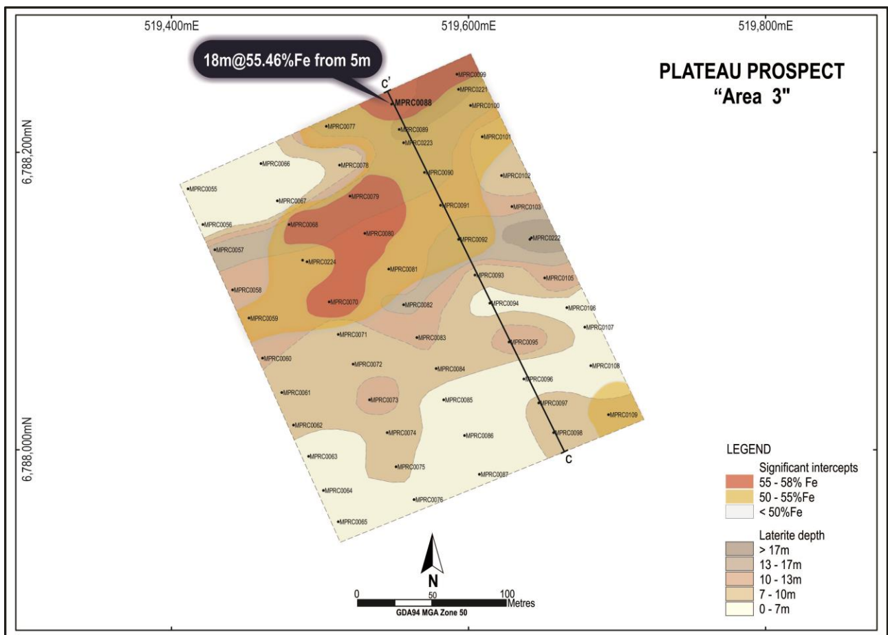
Figure 6: Area 3 showing the location of the drill holes, the distribution of the laterite depth and contour lines for the iron grades. The black line shows the location of the cross section shown in Figure 7 below.
