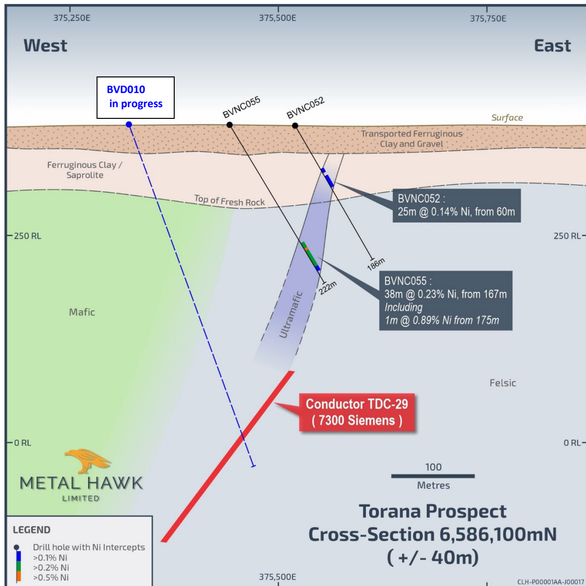
Figure 2. Torana cross-section showing planned drillhole and conductor TDC_29
