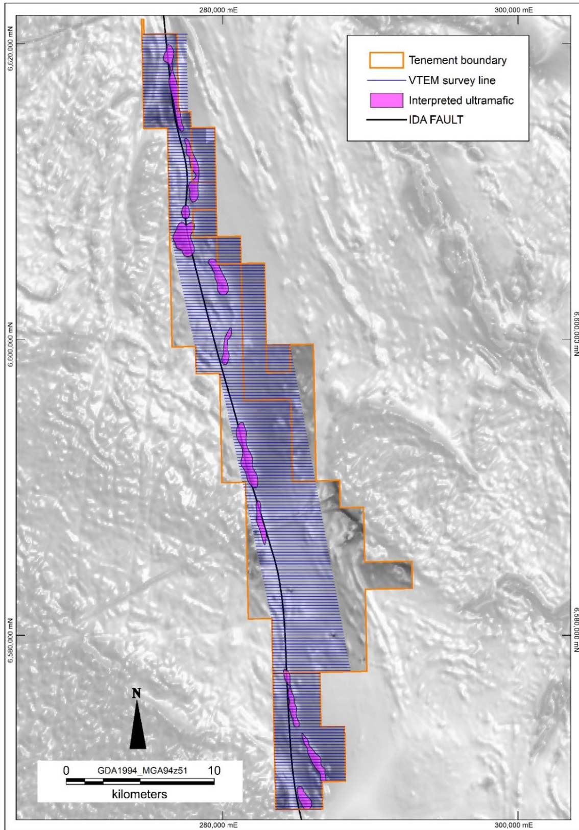
Figure 2. Yarmany Project showing planned VTEM survey lines over aeromagnetic image
