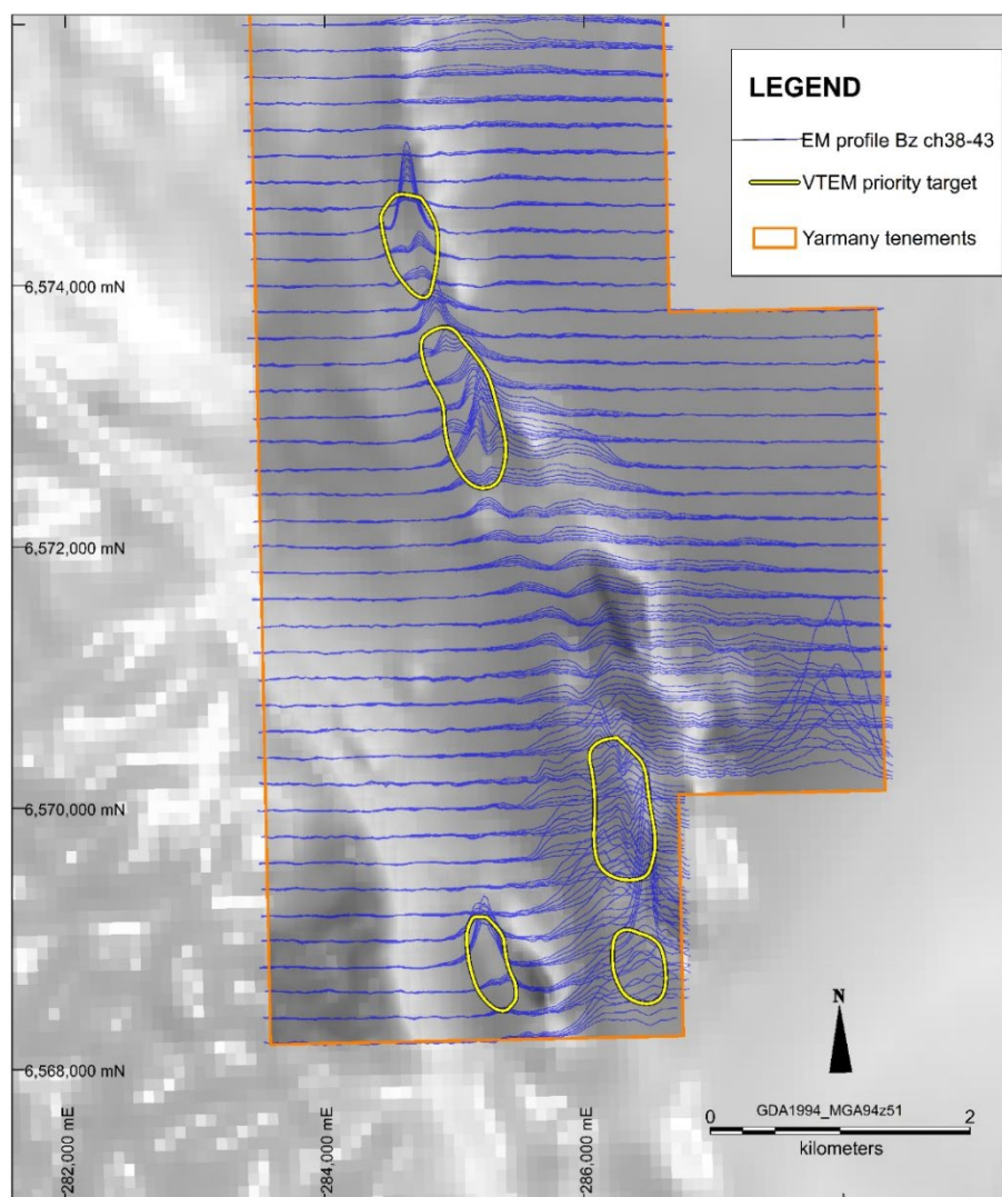
Figure 4. Yarmany southern tenement area showing conductive target areas (yellow) with EM profiles (ch 38-43) over airborne magnetics TMI
