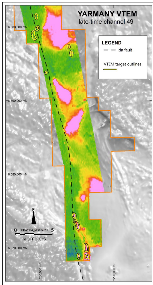
Figure 3b. VTEM targets with late-time image channel 49
