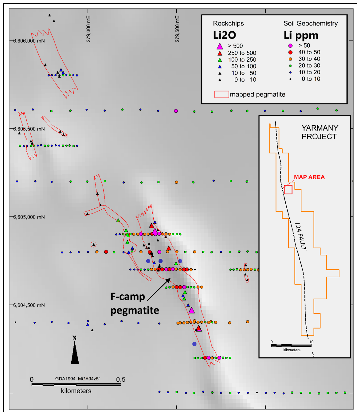
Figure 1. Yarmany Project F-camp prospect surface geochemistry
