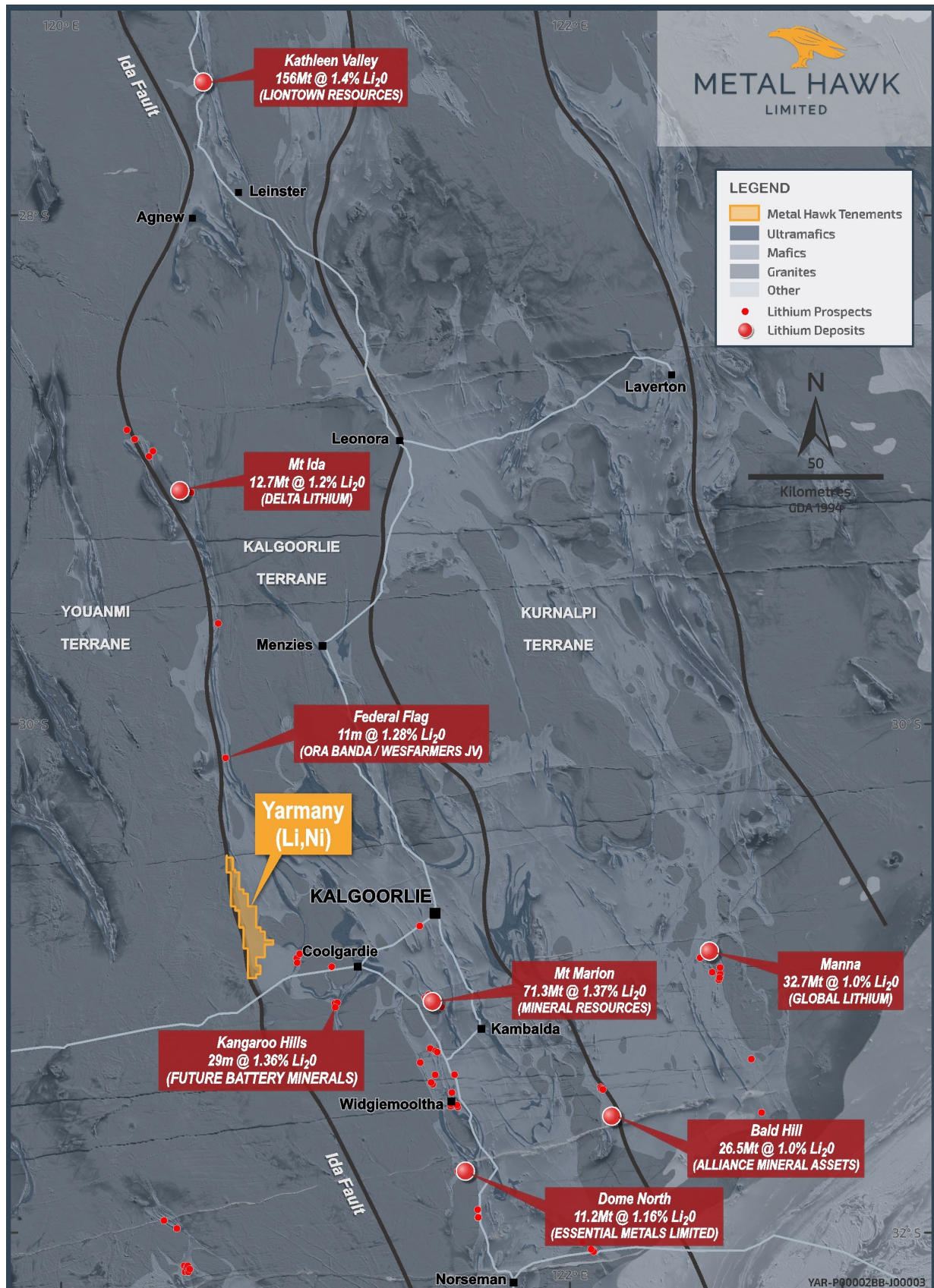
Figure 2. Yarmany Project in relation to other lithium projects in the Kalgoorlie Terrane
