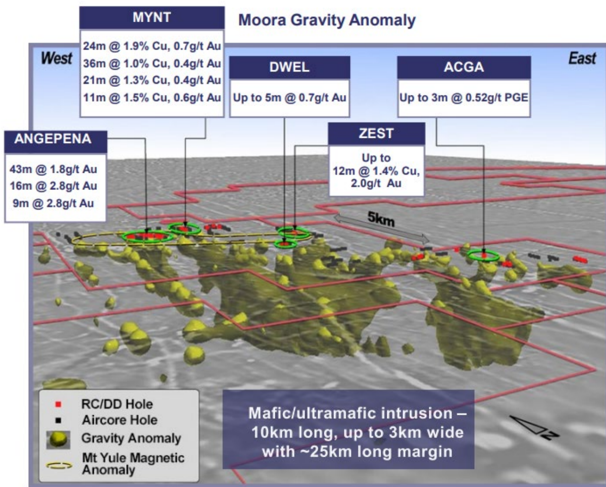
Figure 3 - Moora Gravity Anomaly: Key Exploration Results and Targets.
