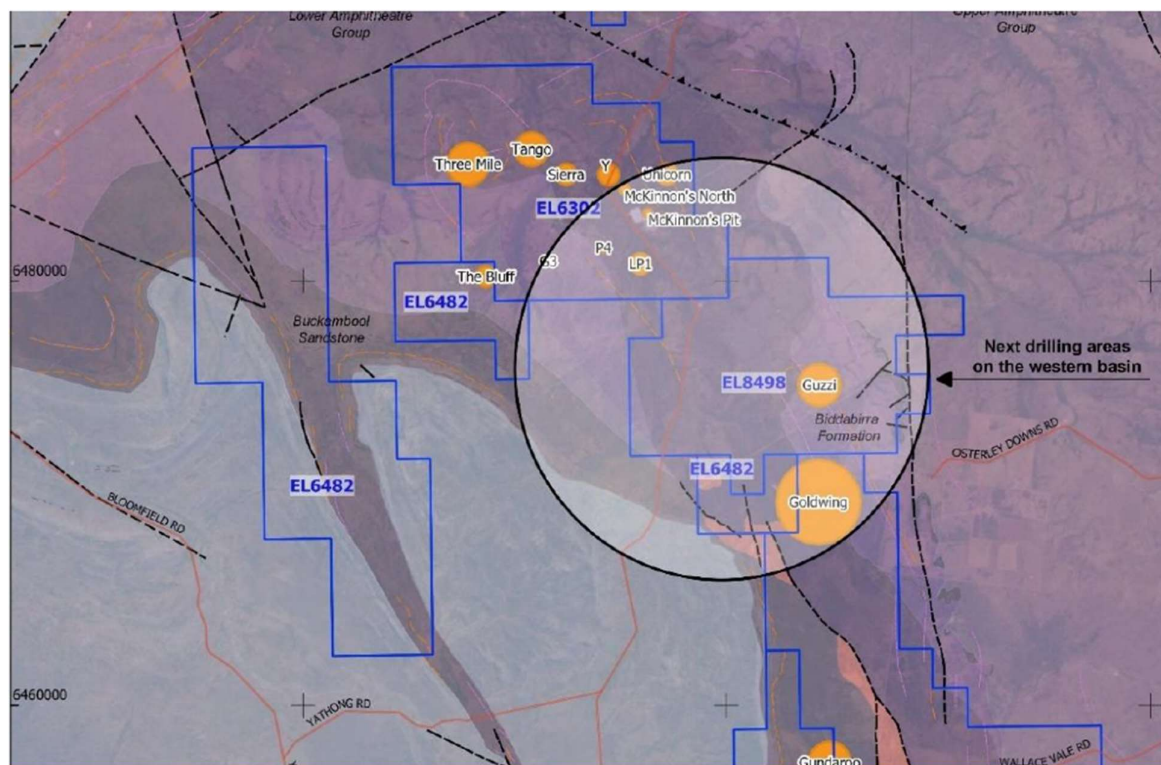
(Figure 7 – Gold exploration targets in the McKinnons mine area, north of Wonawinta)
