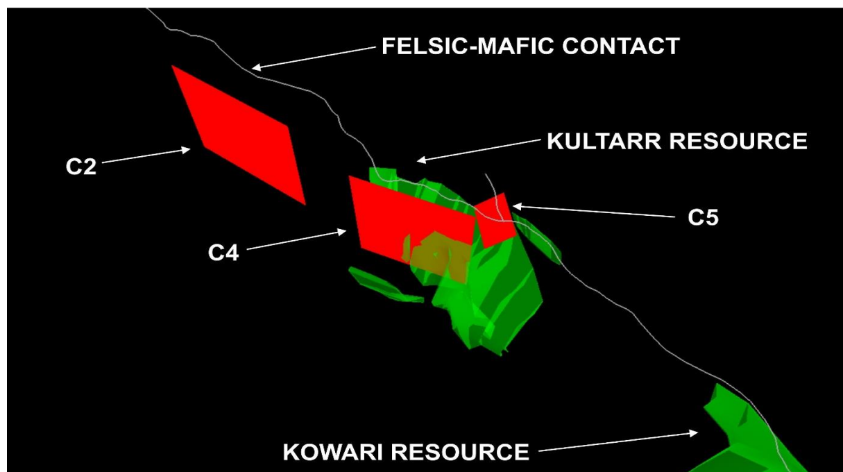
Figure 3: 3D model view of the C2, C4 and C5 Conductors. Also plotted is the resource at Kultarr, the resource at Kowari and the felsic-mafic contact.
