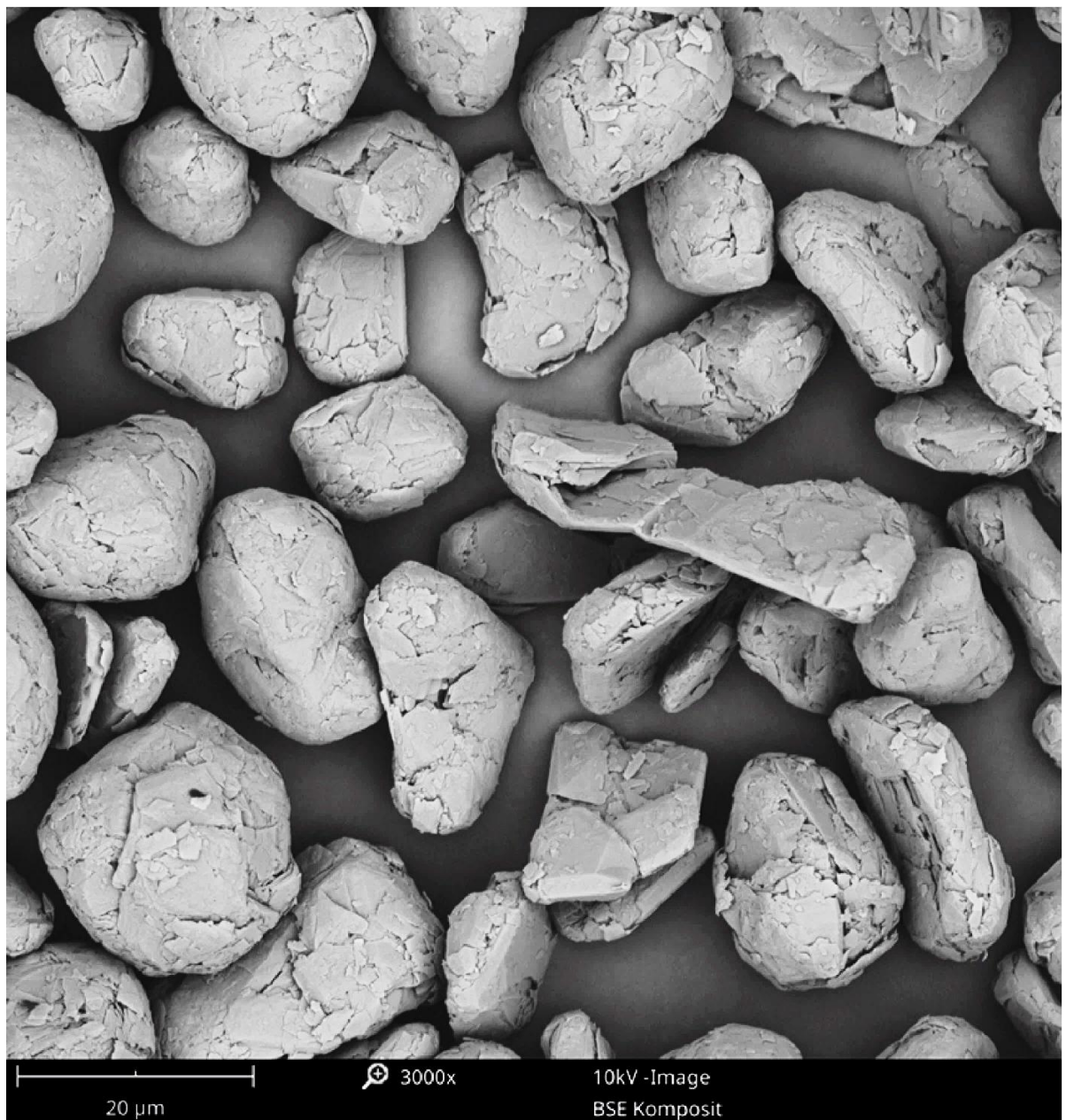
Figure 17: SEM image of reference material Ref 17; magnification 3,000x
