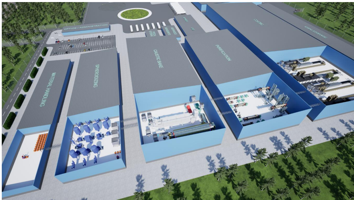
Figure 24: Processing areas for one module of the BAM Facility, arranged in a parallel configuration
