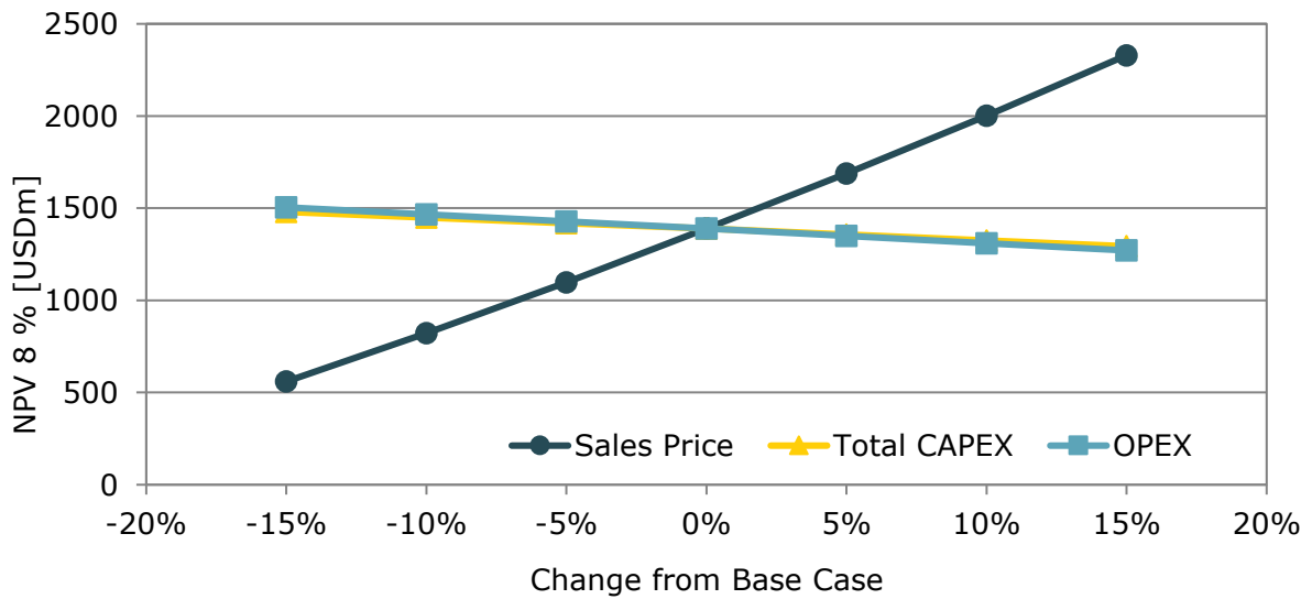
Figure 37: NPV sensitivity to key economic parameters
