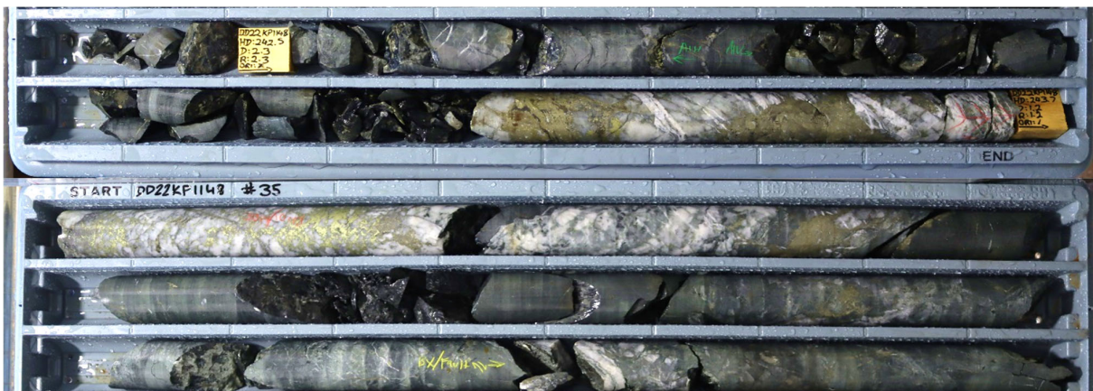
Figure 1: DD22KP1148 with quartz-pyrite-chalcopyrite veining at approximately 243m downhole.
