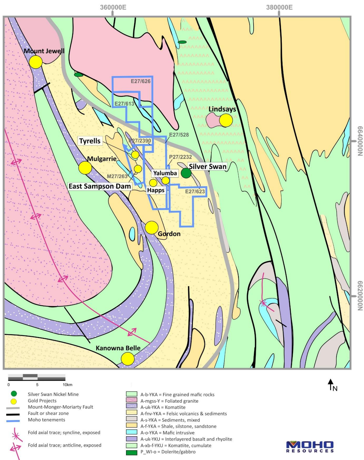
Figure 1: Moho tenement interest in relation to regional geology of Silver Swan North Project
