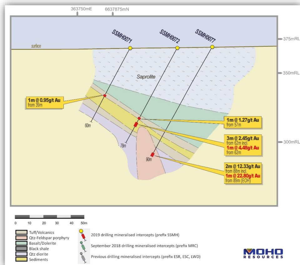
Figure 6: East Sampson Dam September 2019 Drilling, Section 9a looking NW
