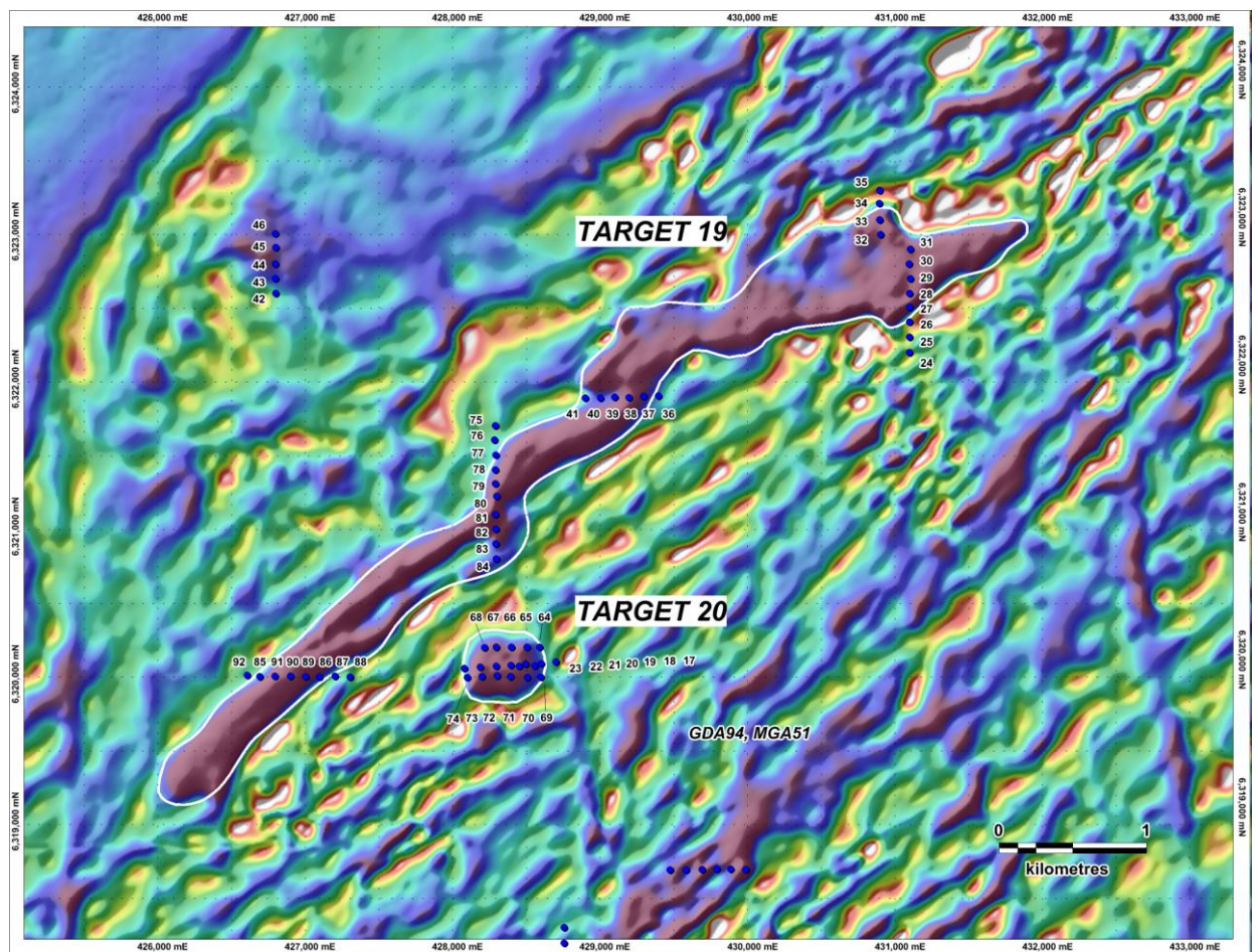
FIGURE 1: Aeromagnetic image showing location of aircore drill holes over Targets 19 and 20.
