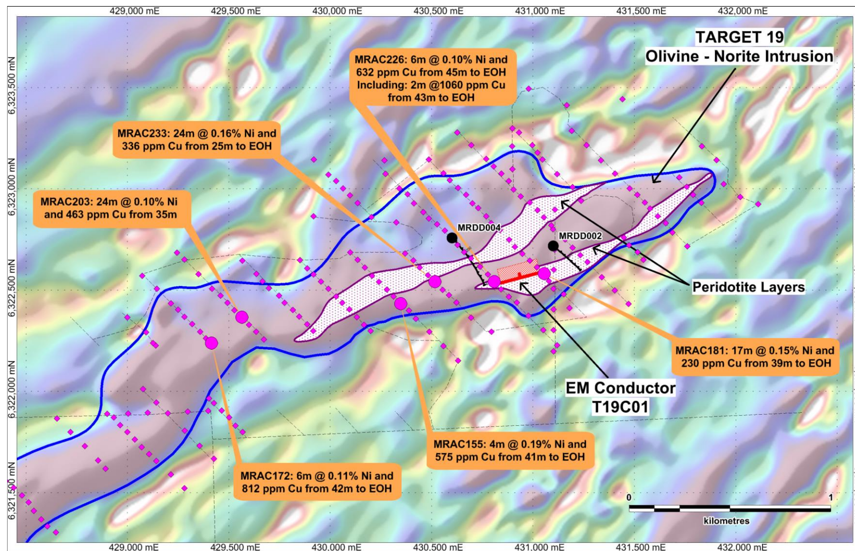
FIGURE 3.0 – Aeromagnetic image showing position of peridotite zone and location of EM Conductor Pink dots represent aircore drillhole locations and black dots represent diamond hole locations.
