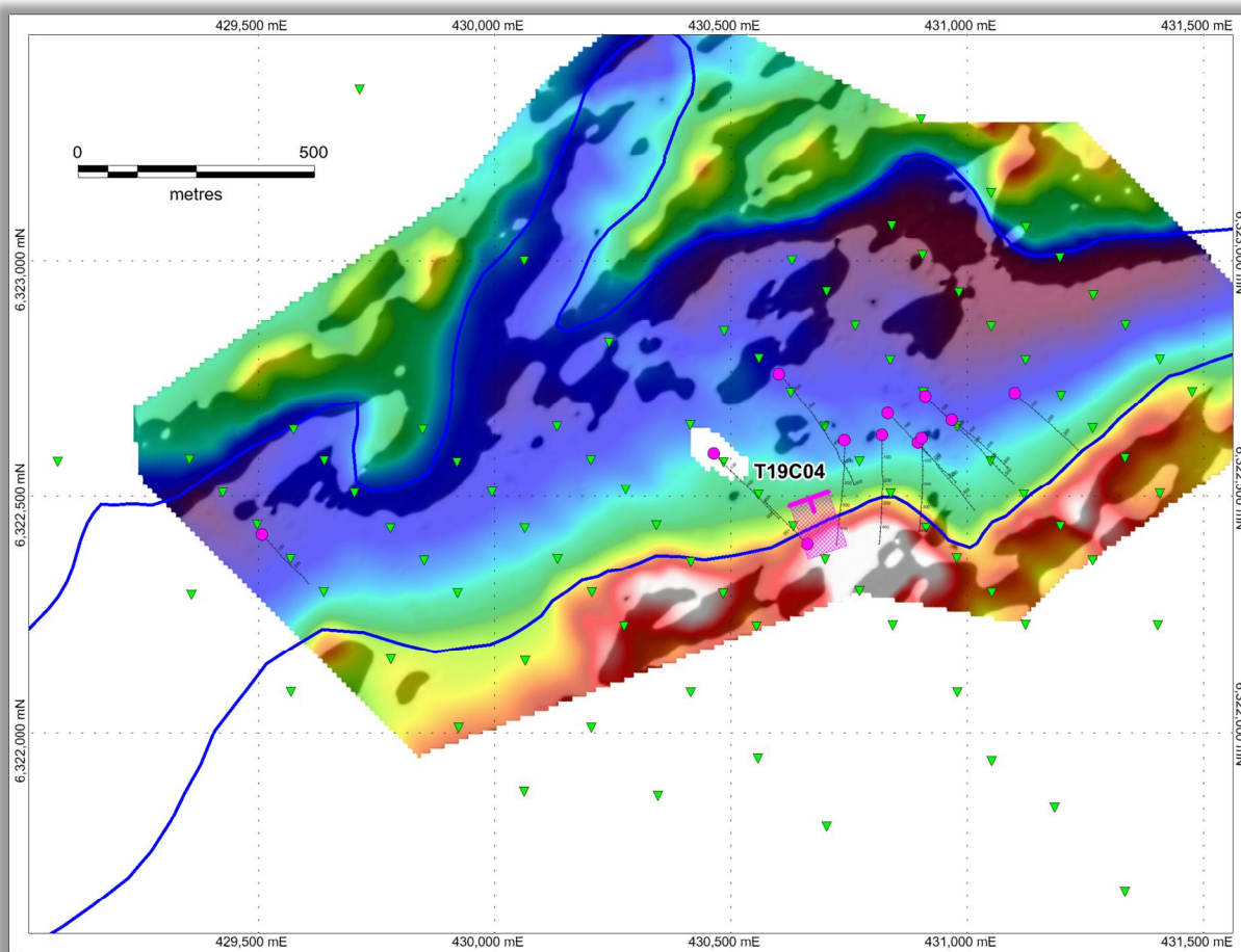
Figure 4.0 – Plan showing location of bullseye magnetic anomaly (white in colour) in relation to existing diamond holes, the flexure in the SE contact and the new fixed loop EM conductor T19C04.
