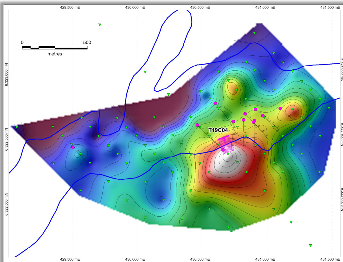
Figure 2.0 – Plan showing new AMT phase anomaly (10 Hz with 1 degree contours) together with the location of the new fixed loop EM conductor T19C04 and existing diamond holes. Red and white colours indicate more highly conductive material while the green and blue colours indicate less conductive. The stronger conductor target is located approximately 100m down plunge beneath the existing diamond drilling.
