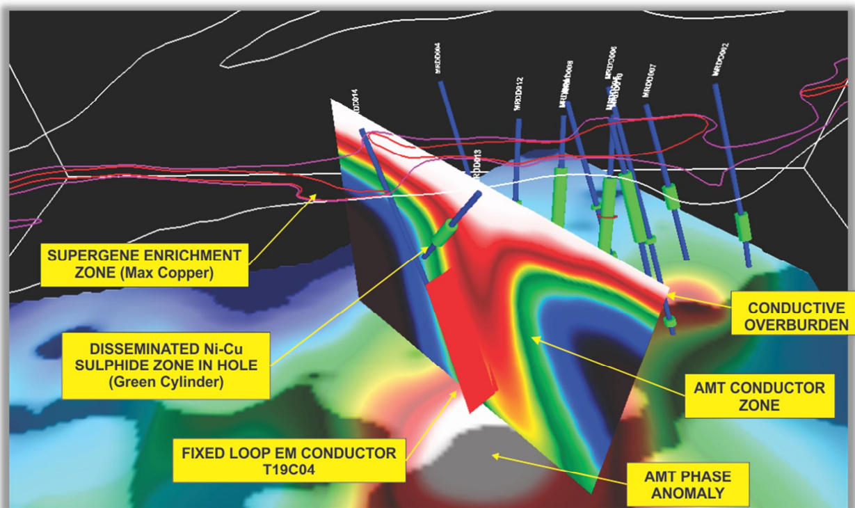
Figure 1.0 – 3D perspective view showing several key elements that make up this new priority drill target. They include new fixed loop EM conductor T19C04, cross section 45900N highlighting AMT conductor zone and new AMT phase anomaly. The phase anomaly, shown in white-red, is indicating an area of higher conductance positioned down plunge from existing drilling.
