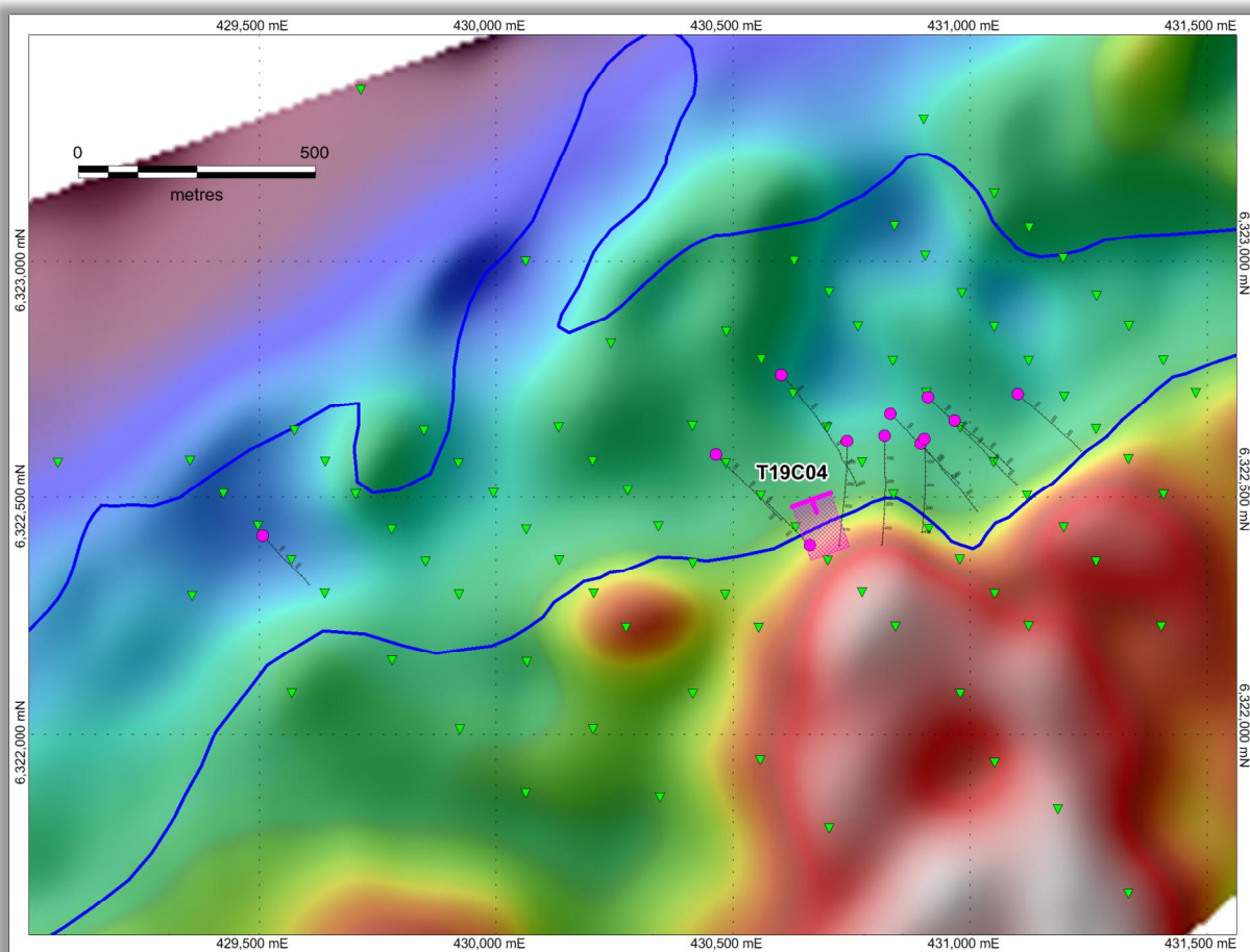
Figure 5.0 – Plan showing location of gravity anomaly (red-white in colour) in relation to existing diamond holes, the flexure in the SE contact and the new fixed loop EM conductor T19C04. The area is quite complex and made up of several gravity anomalies some of which will be related to the geology outside the intrusion.
