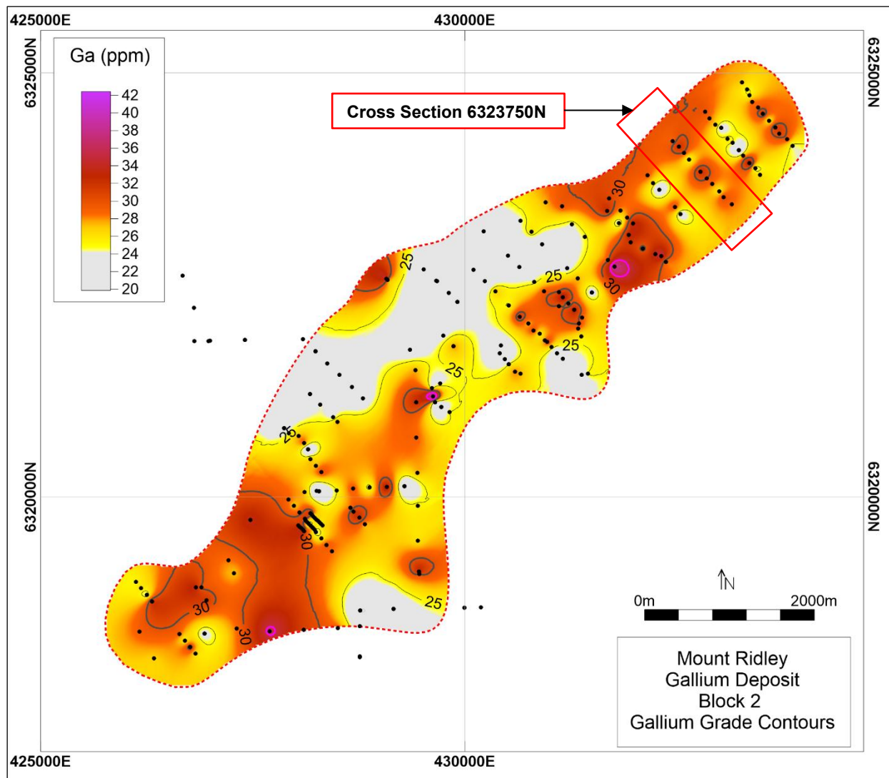
Figure 5 – Block 2 Gallium Average Grade Contours
