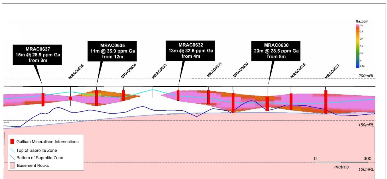
Figure 6 – Block 2 Cross Section 6323750mN highlighting Ga Block Model Grades
