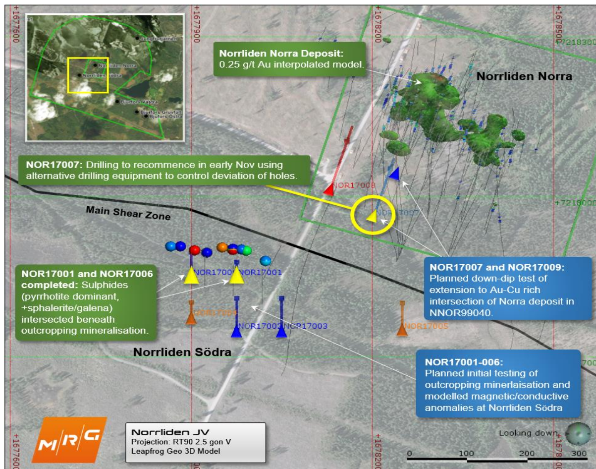
Figure 2. Drillholes completed at Norrliden Södra in September 2017 (yellow), and location of initial drillhole attempted at Norra. Deviation of the hole NOR17007 due to strong foliation in the rock was significant enough to compromise the effectiveness of the drillhole. Drilling equipment better suited to controlling the hole in these conditions will be brought in to recommence the hole in early November.
