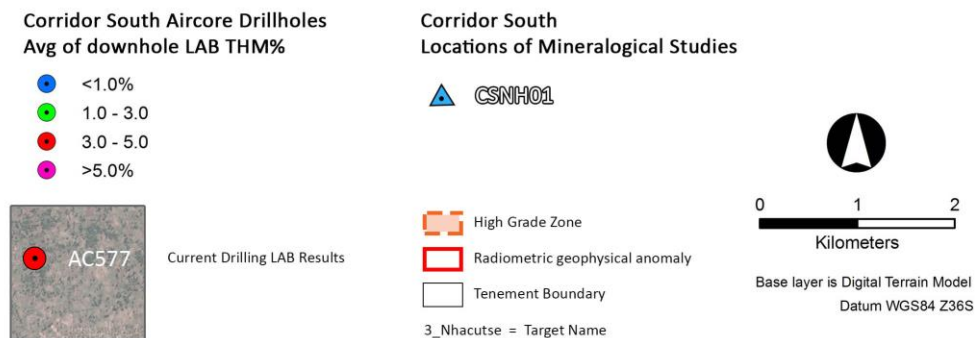
Figure 7: Mineralogical samples in relation to Phase 2 aircore drillholes and the high grade zones.
