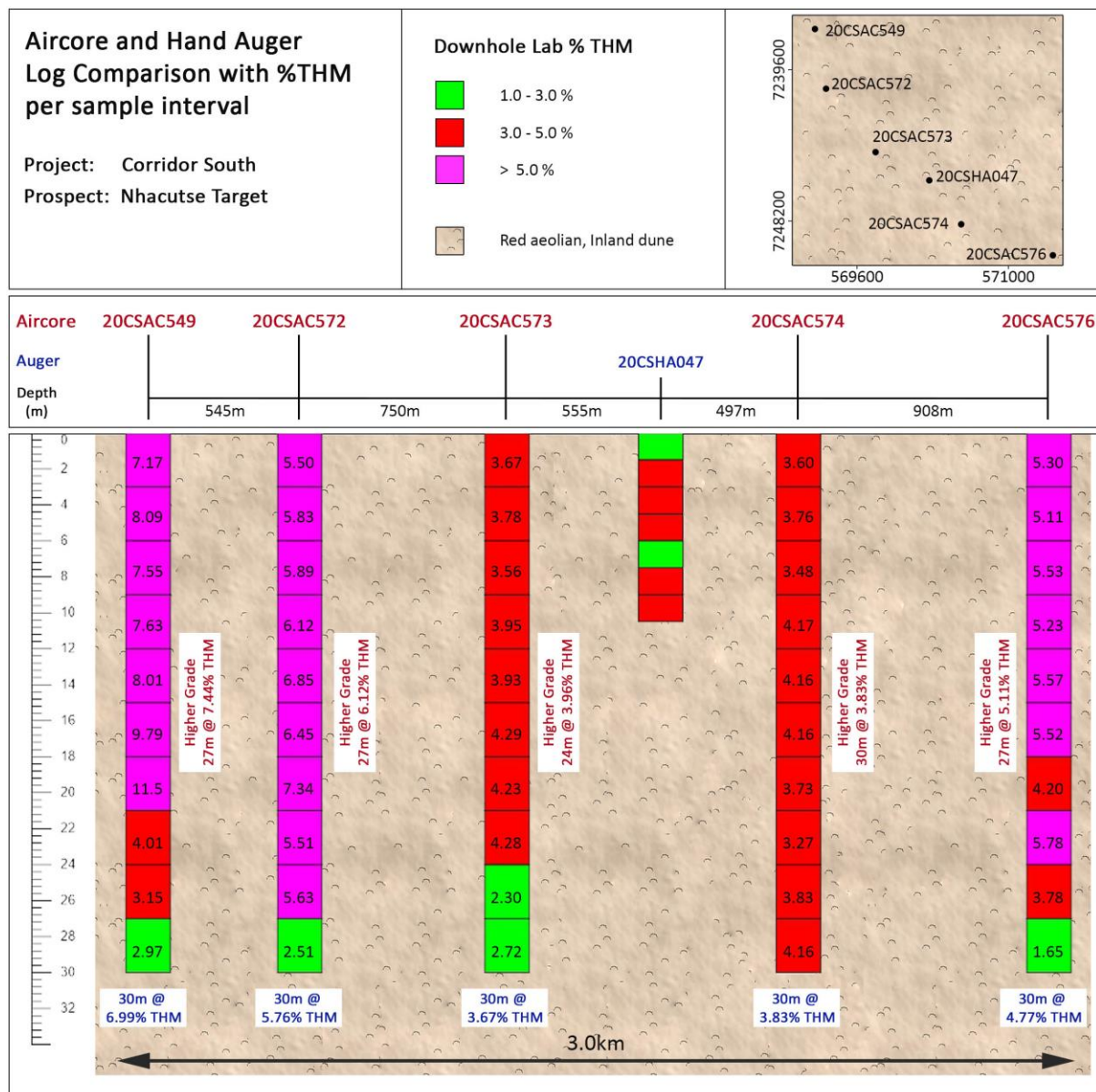
Figure 5: Cross section showing aircore and hand auger holes drilled between the towns of Nhacutse and Bungane, sections shows the link in grades, as well as the high THM grades in the Nhacutse High Grade zone. Section shows % THM results for each sample intersection, the average of the entire drillhole as well as where applicable a higher grade cut (using a lower cut-off of 3% THM) is shown. Note: The focus of this section is to show sample by sample downhole assays. Due to the vertical exaggeration required to do this, the surface profile is not shown.
