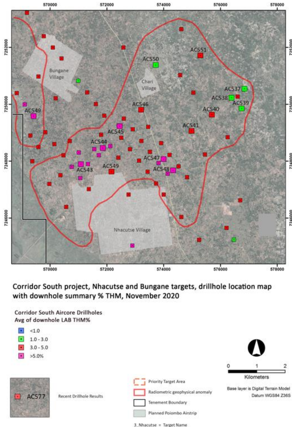
Figure 7. Aircore drillhole locations for Nhacutse High Grade Zone and Bungane Target showing summary data for THM% assay grades.
