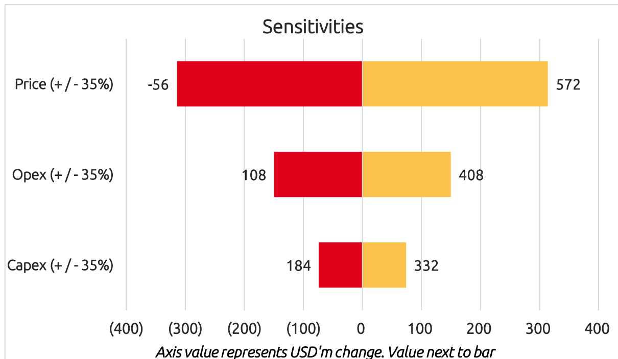
Figure 7: Sensitivity analysis
