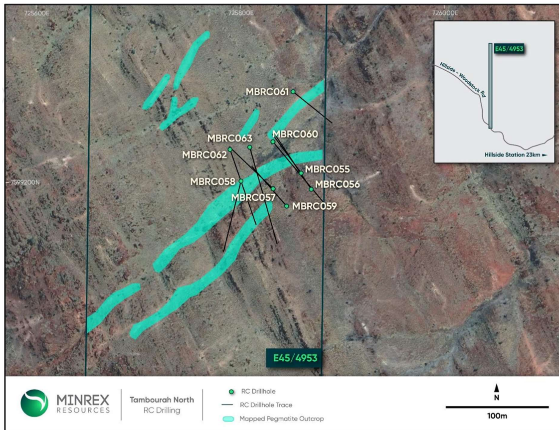
Figure 2 – Tambourah North RC Drilling
