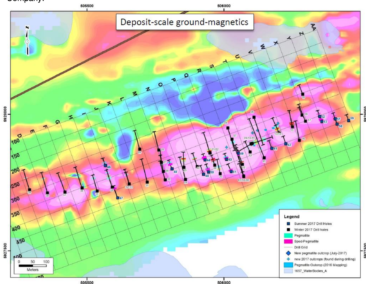
Figure 1: Diamond drill hole location map and pegmatite outcrops identified at the Cancet Lithium Project
