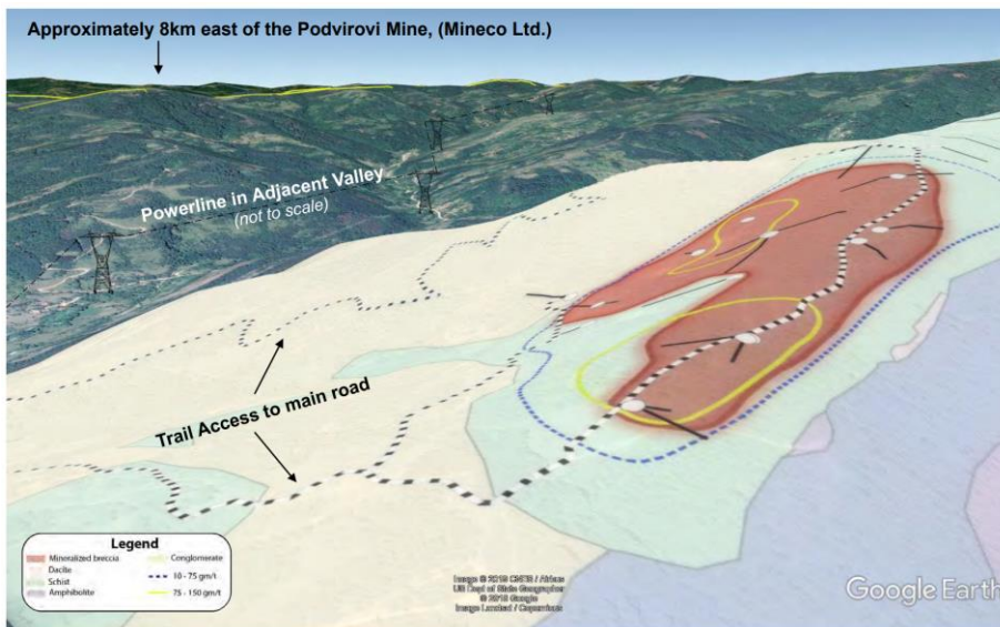
Figure 11 and 12: Tlaminu Gold Project infrastructure layout map and road access diagram
