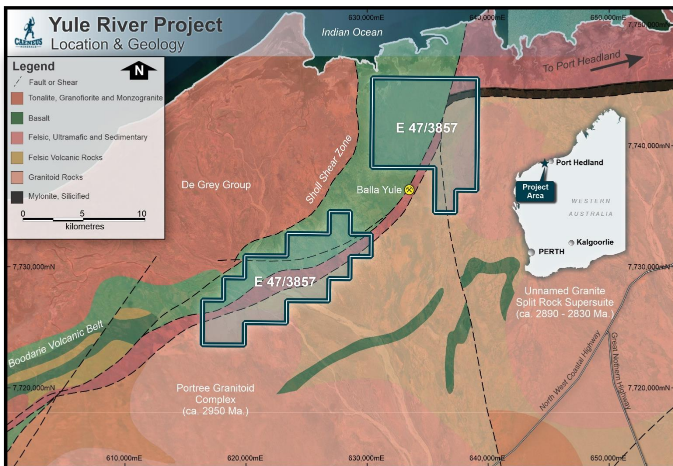
Figure 1: Yule River Project Location & Geology
