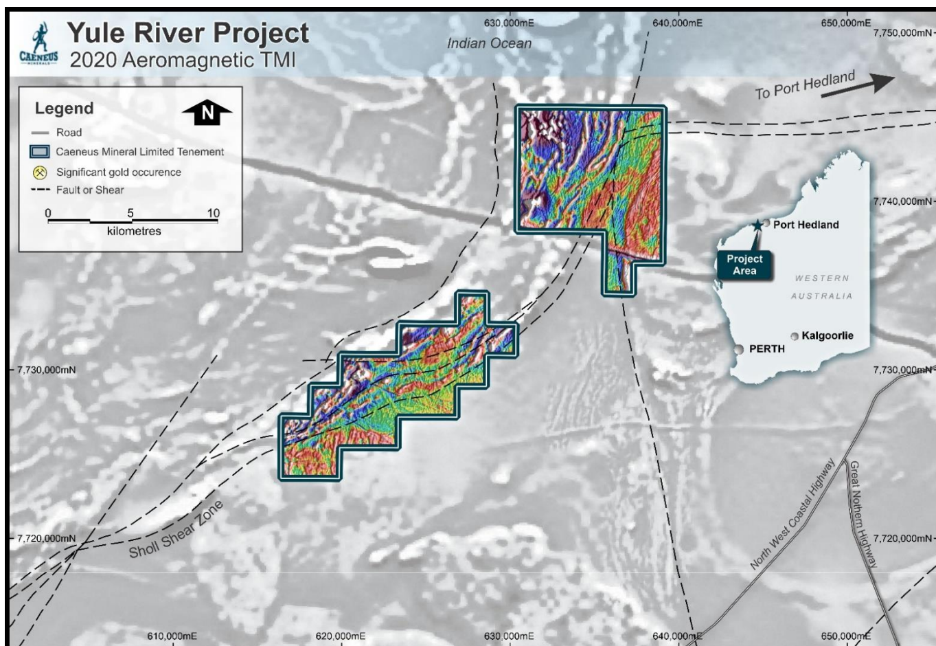
Figure 2: Yule River Project TMI
