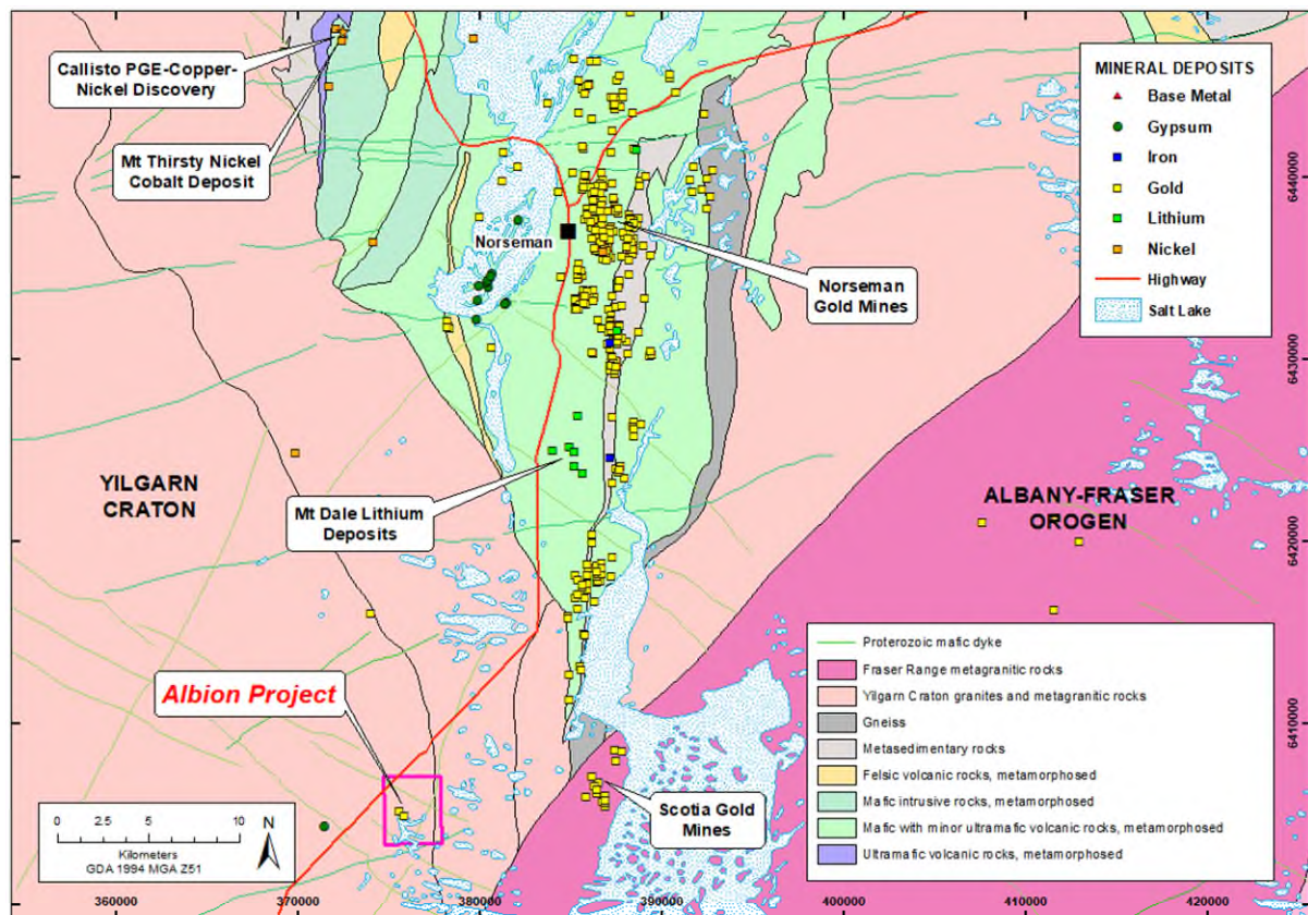
Figure 1: Regional interpreted geology map of the Norseman area showing significant mineral deposits and the location of the Albion project.
