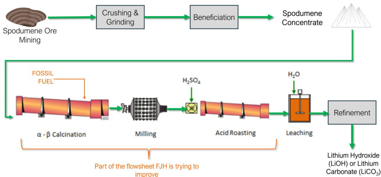
Figure 1: Simplified flowsheet for Lithium production from hardrock spodumene ore source showing the phases that the FJH process will target for improvements.
