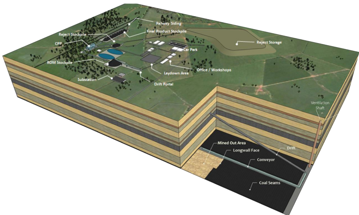
Figure 2- Conceptual Drawing of Lochinvar Mine, Process Plant and Surface Infrastructure
