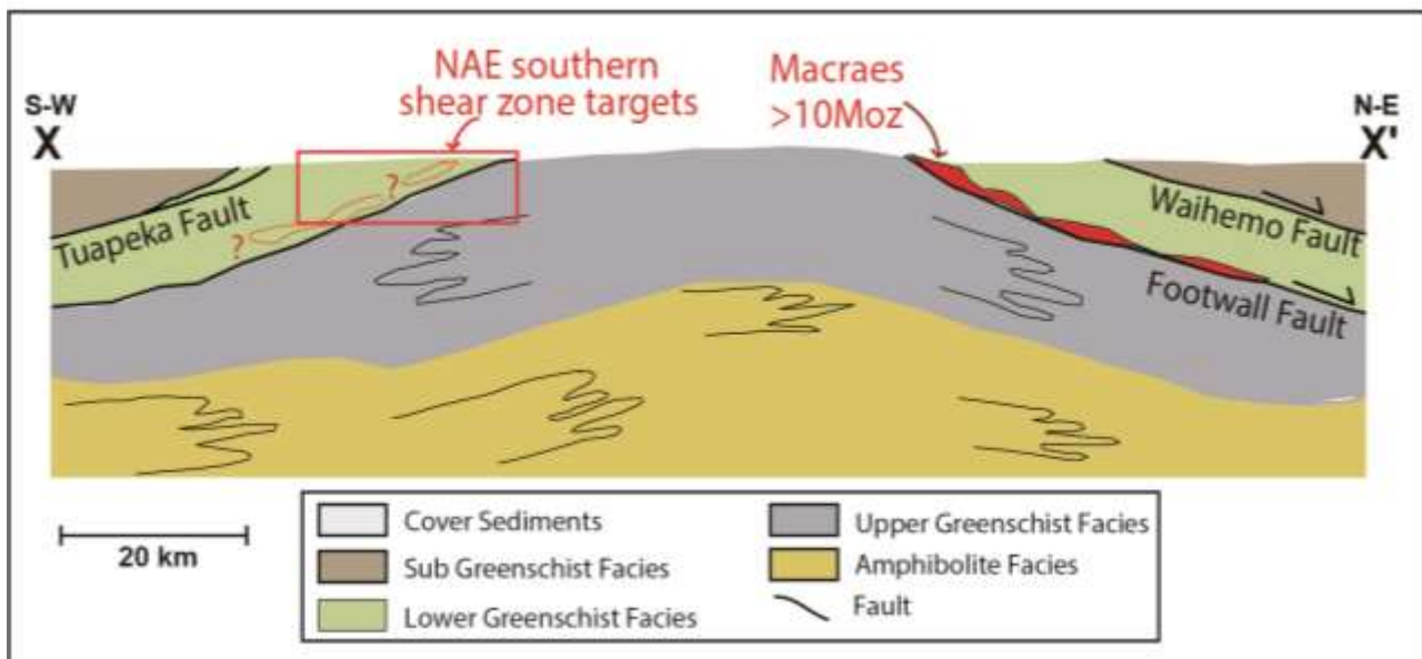
Figure 6 - Geological Cross section - Otago Schist Belt & Southern Shear Zone Gold Exploration Targets
