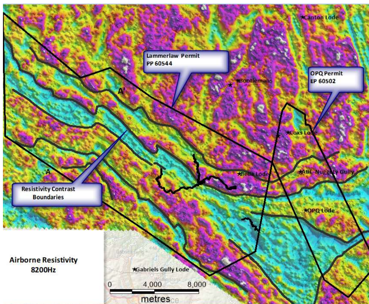
Figure 3 - Target areas on airborne resistivity
