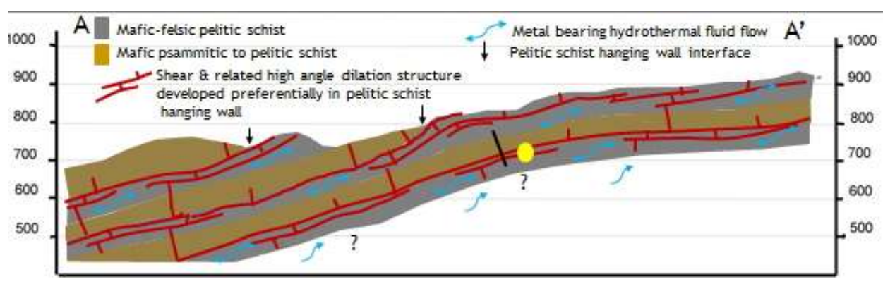
Figure 4 - Conceptual cross section Lammerlaw permit
