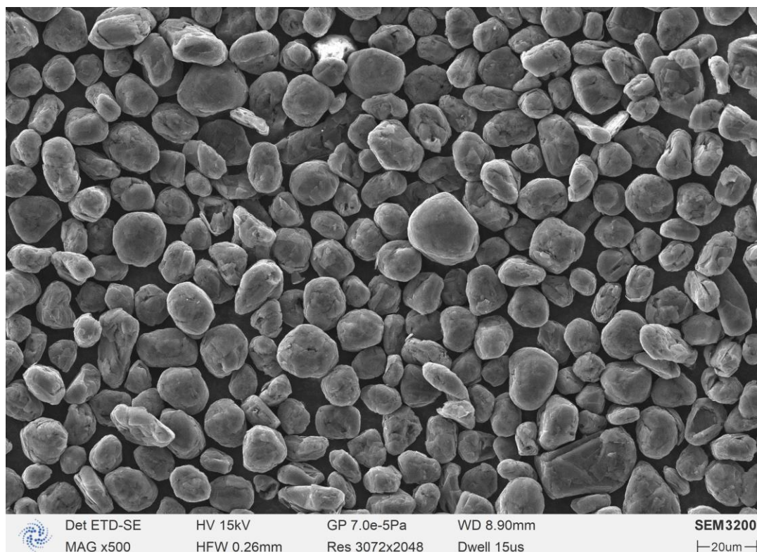
Figure 1: Scanning Electron Microscope image of CSPG produced from Upgraded Malingunde Concentrate showing conventional potato-shaped particles
