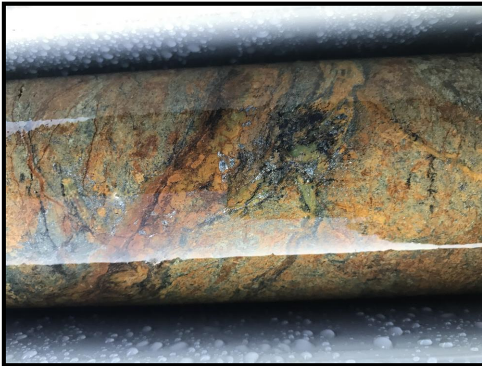
Figure 2 – Oxidised ultramafic in drill core (below surface gossan) (NRDD005) testing down-dip of the Dease Gossan (27.8m).
