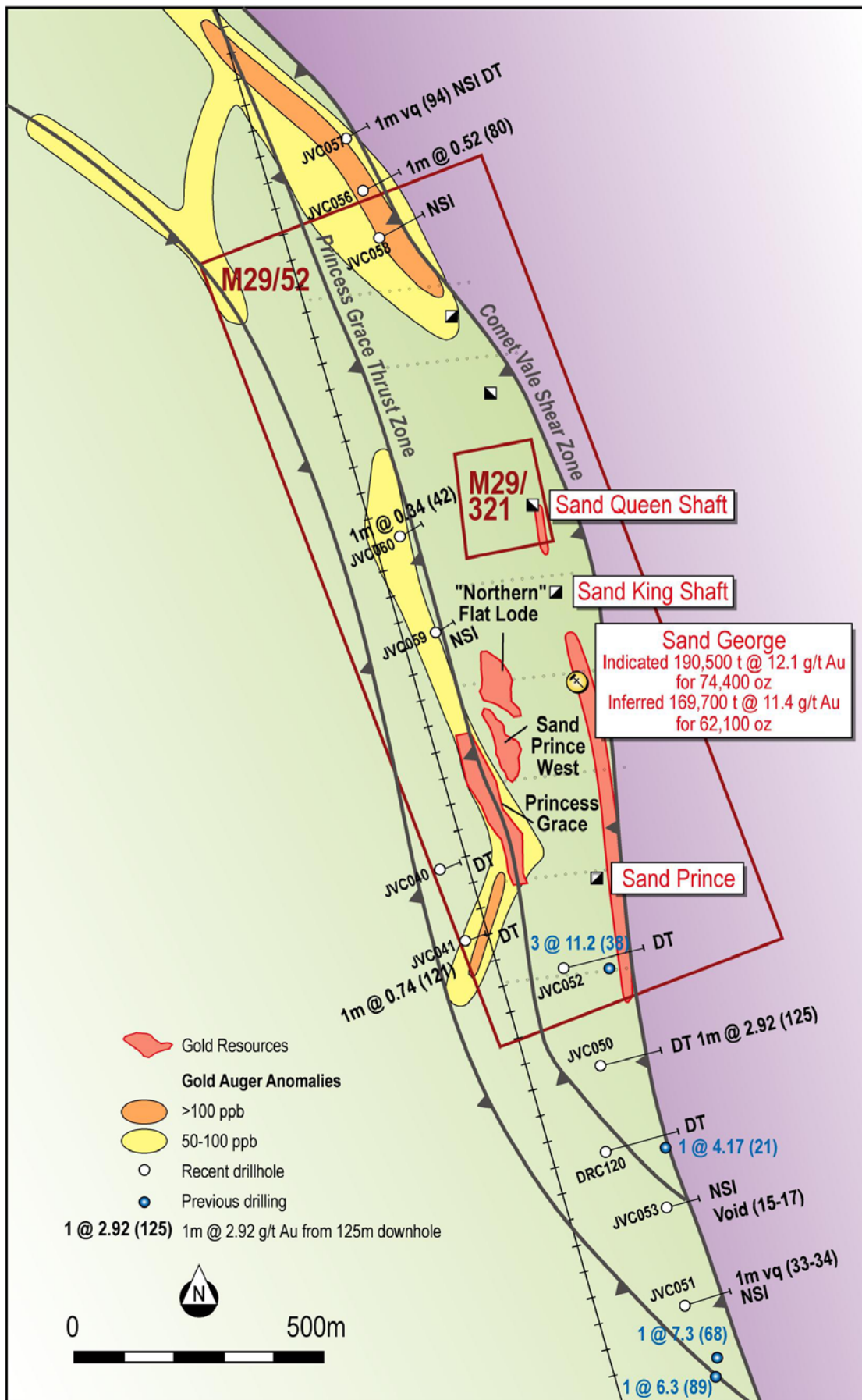
Figure 3 Plan of Current Exploration Program. Proposed holes have results from recent RC precollar, then followed by "DT".
