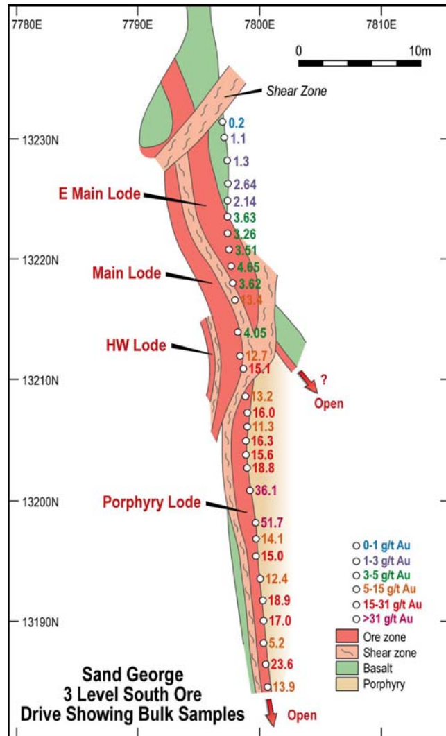
Figure 2 Plan showing development drive bulk samples on the 3 Level.
