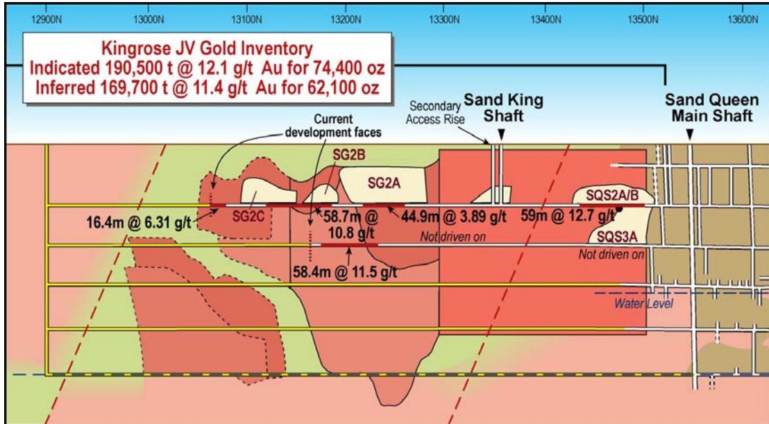
Figure 1 Long section looking west, Sand Queen Gold Mine showing stope outlines and averaged development bulk sampling at end of August 2007.
