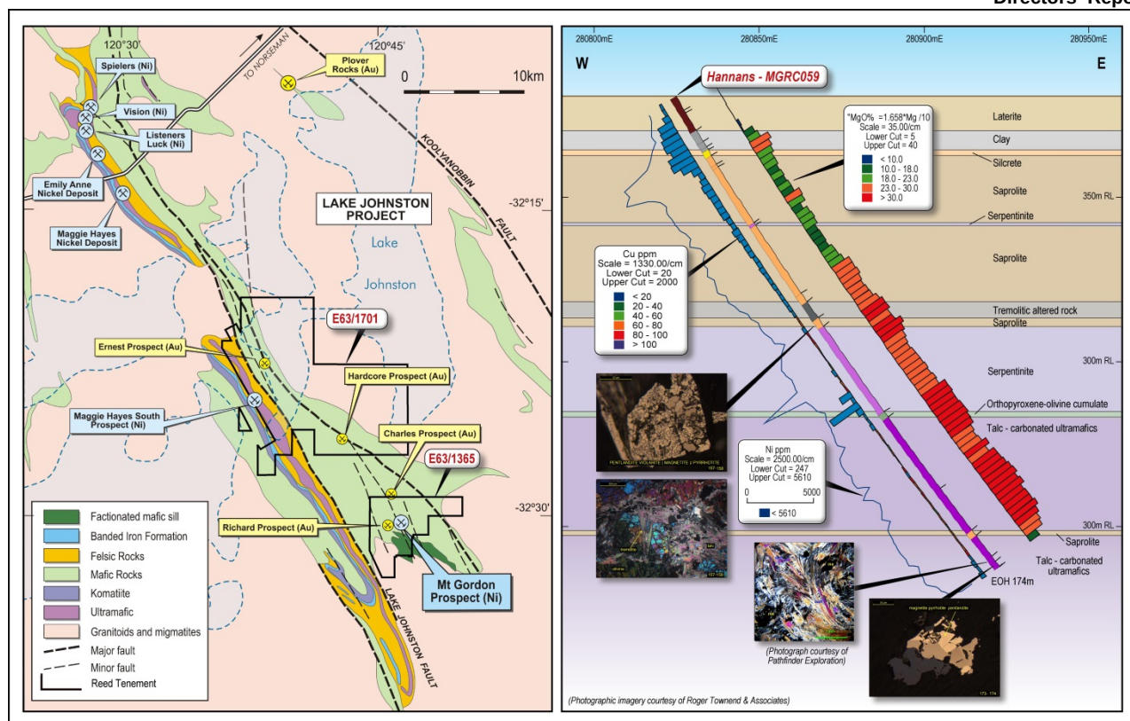
Figure 1. Tenement Plan on Interpreted Geology
