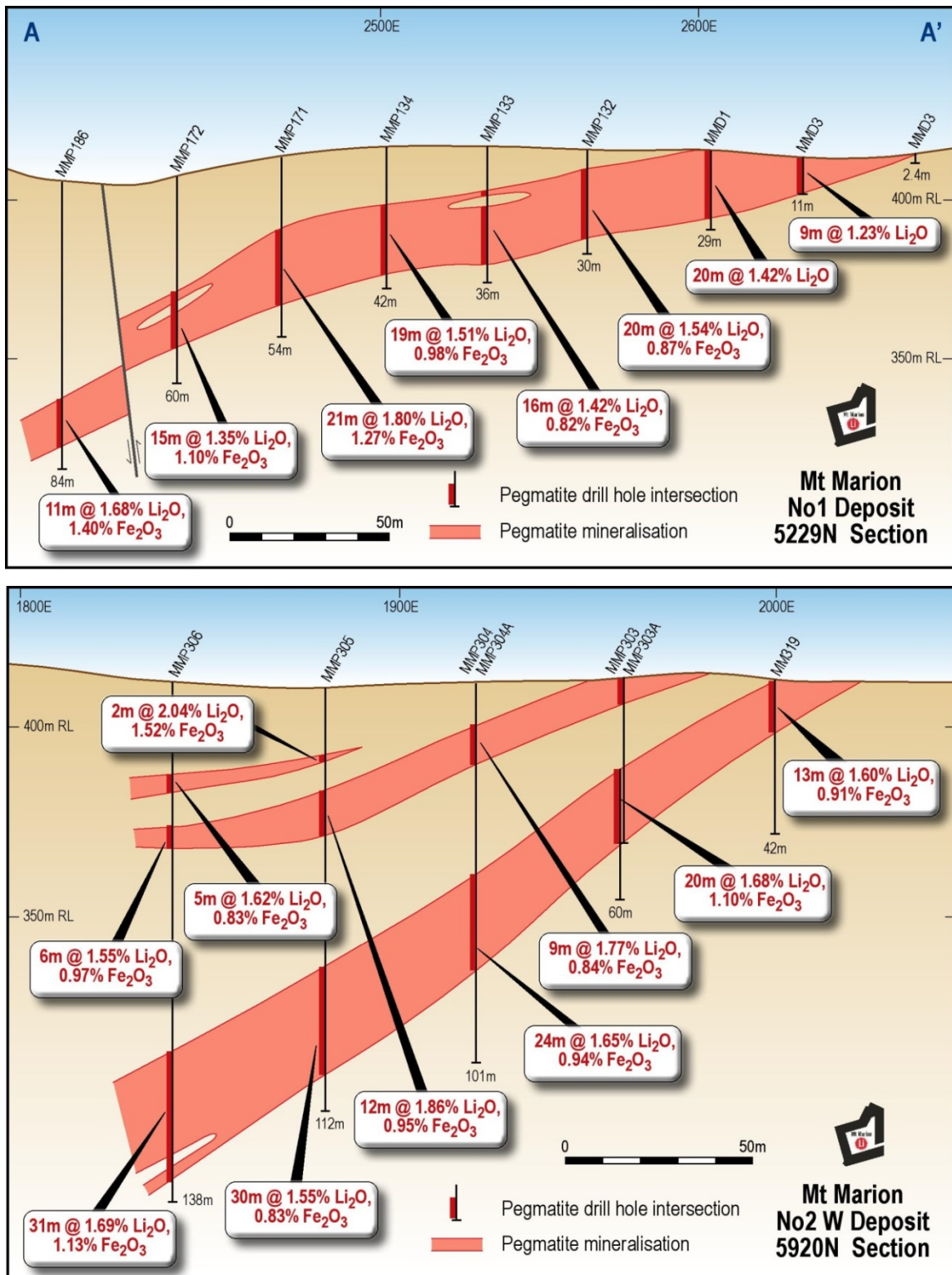
Figure 4 and 5 Representative Cross Sections with Lithium Intercepts
