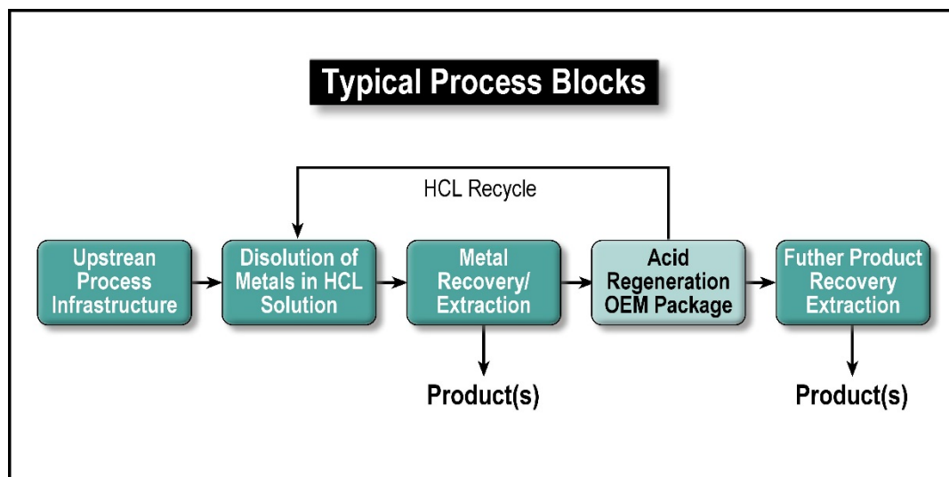
Figure 2. Neomet Proprietary Acid Regeneration Technology Process Model
