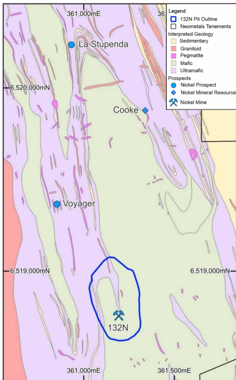
Figure 2 - Geology around 132N (pit outline shown in blue). Mineralisation on the ultramafic-basalt contact is intensified on the axis of the parasitic syncline on the west limb of the Widgiemooltha Anticline
