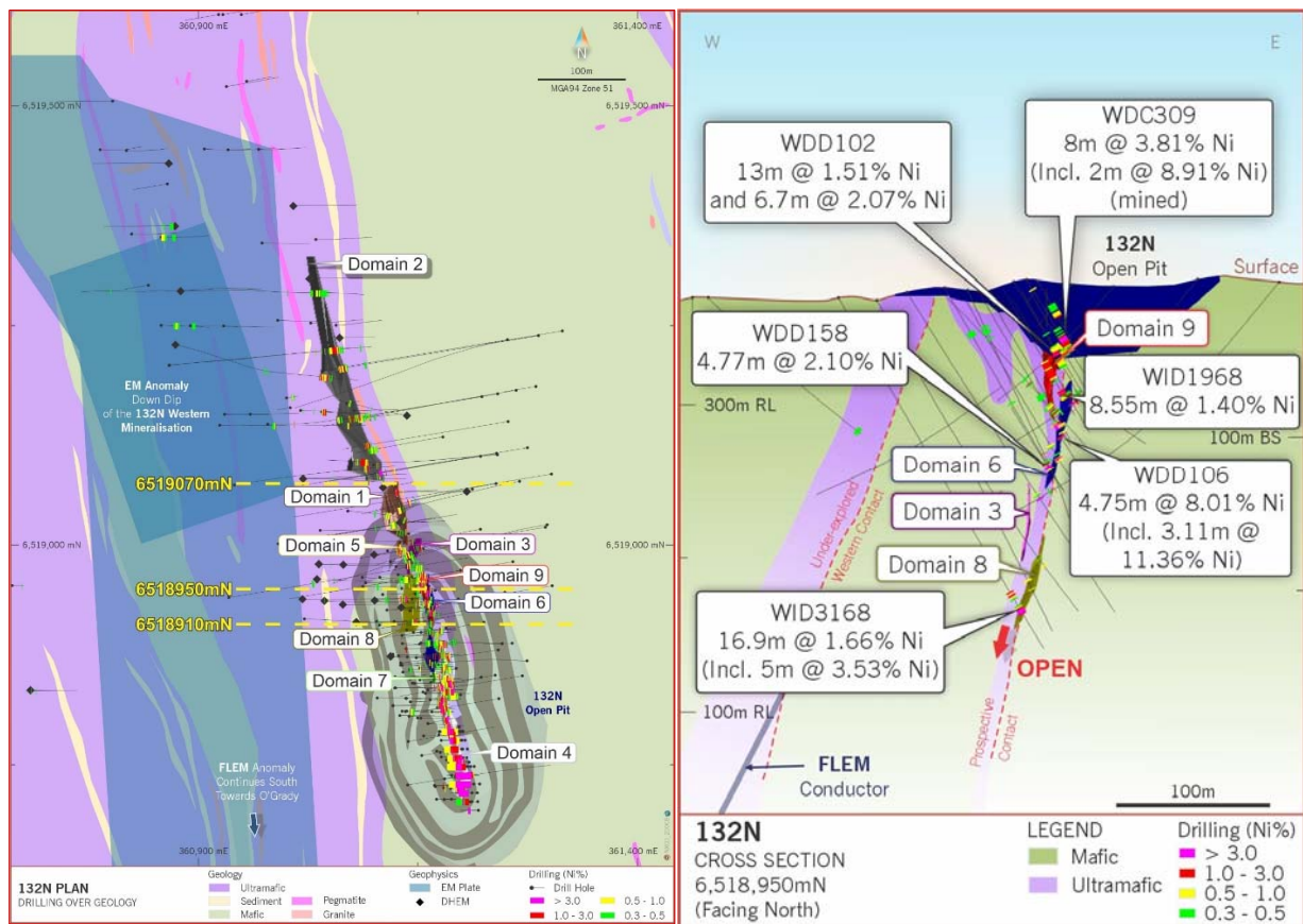
Figures 5 &amp; 6 – Plan of the 132N Nickel Mineral Resource with location of sections, and Cross Section at 6,518,950mN
