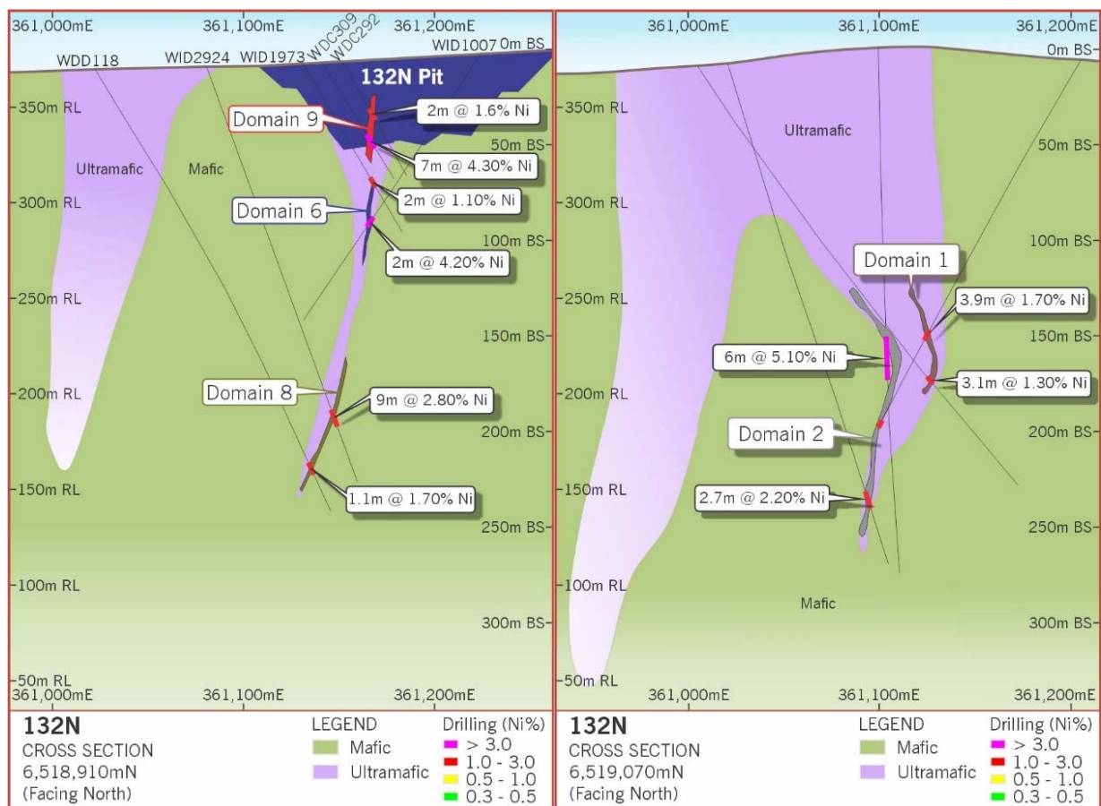
Figures 7 &amp; 8 - Cross Sections at 6,518,910N and 6,519,070N with drill intercepts of the 132N Nickel Mineral Resource
