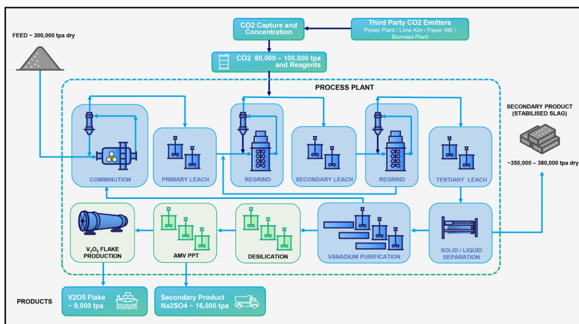
Figure 7 – High level flowsheet of Neometals VRP Technology.
