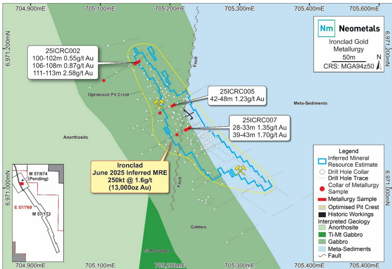
Figure 3: Plan showing location of RC holes 5 used for composites for Ironclad metallurgical test work. Also shown is an outline of the Ironclad Inferred MRE 2 and a representation of the optimised pit shell
