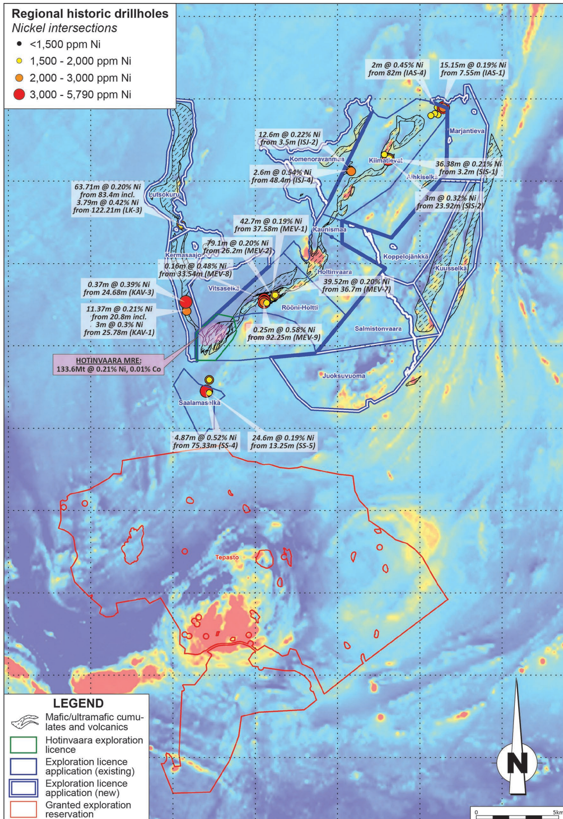
Figure 1. Historic drill hole collar plan and assay highlights over Pulju Project together with new Tepasto Exploration Reservation Area. Background image: total magnetic intensity (Source: GTK, Finland).
