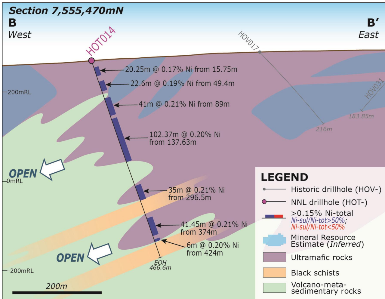
Figure 3. Cross-section B – B' (7,555,470mN) showing down-hole assays of HOT014 and interpreted solid geology. View looking north. True width estimated to be 70-90%.
