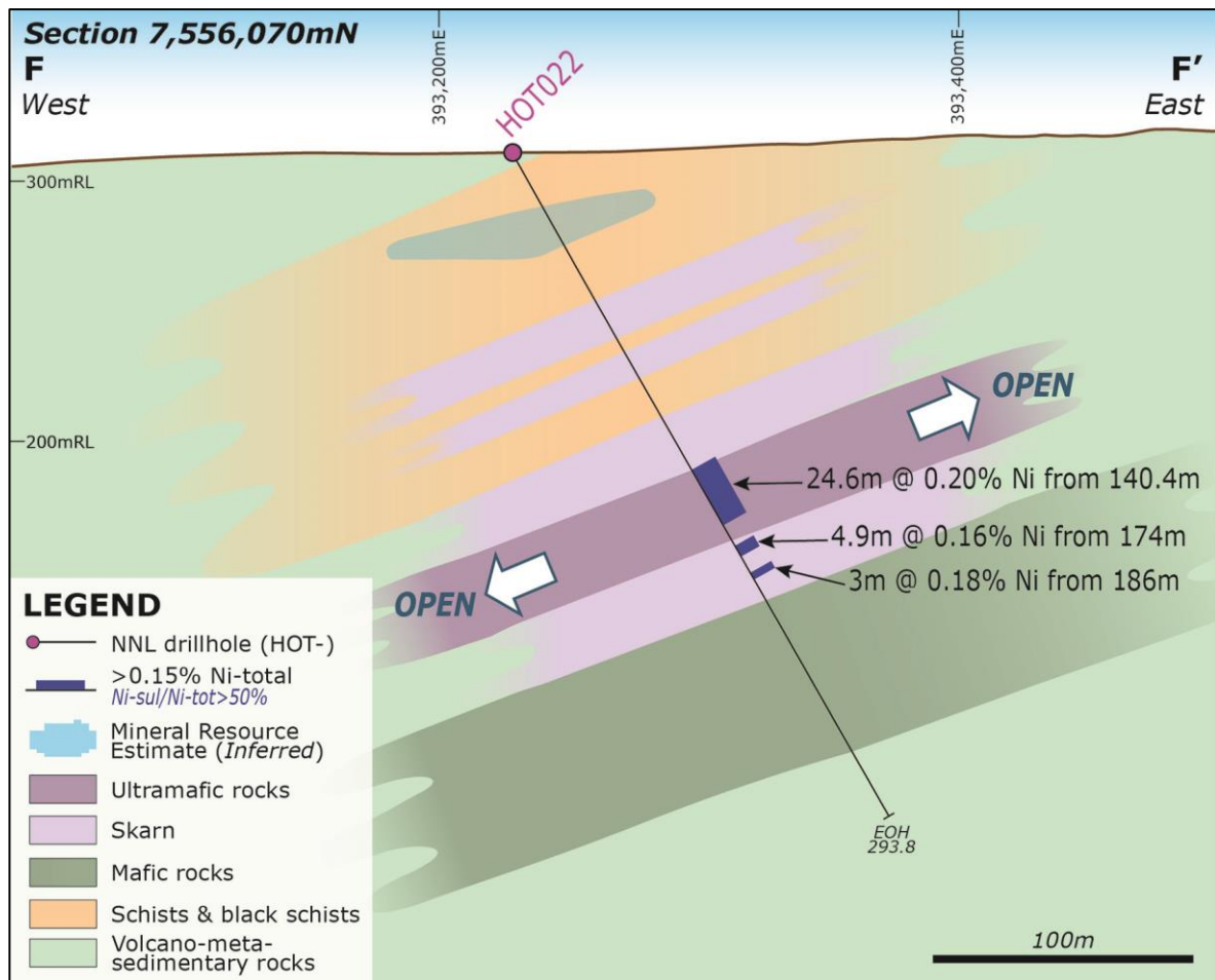
Figure 7. Cross-section F – F' (7,556,070mN) showing down-hole assays of HOT022 and interpreted solid geology. True width estimated to be 70-90%. View looking north.
