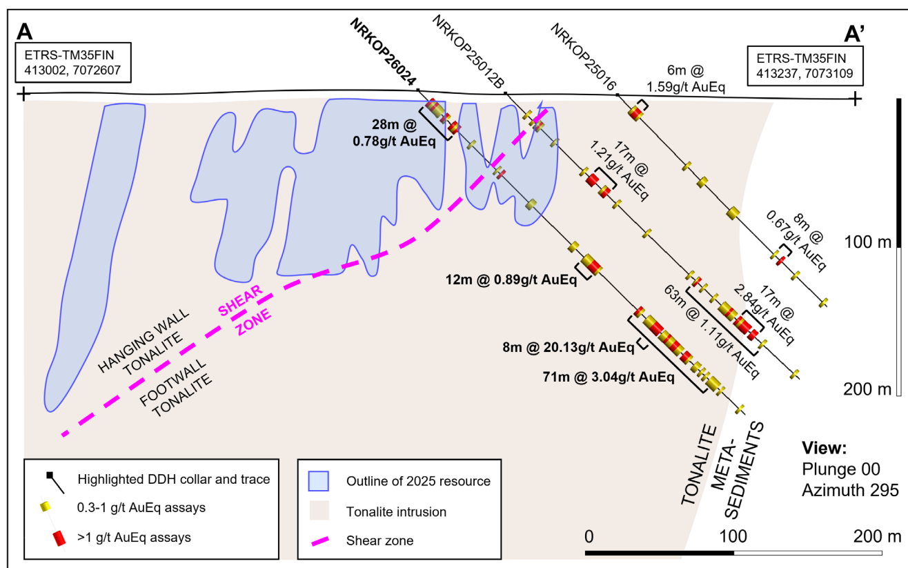
Figure 2: Kopsa cross section showing hole NRKOP26024. The most recent MRE outline and the interpreted extent of the tonalite intrusion are also shown in this 40m thick section view. See Appendix 1 for the drill hole details. Coordinates presented in ETRS-TM35FIN system (EPSG:3067).
