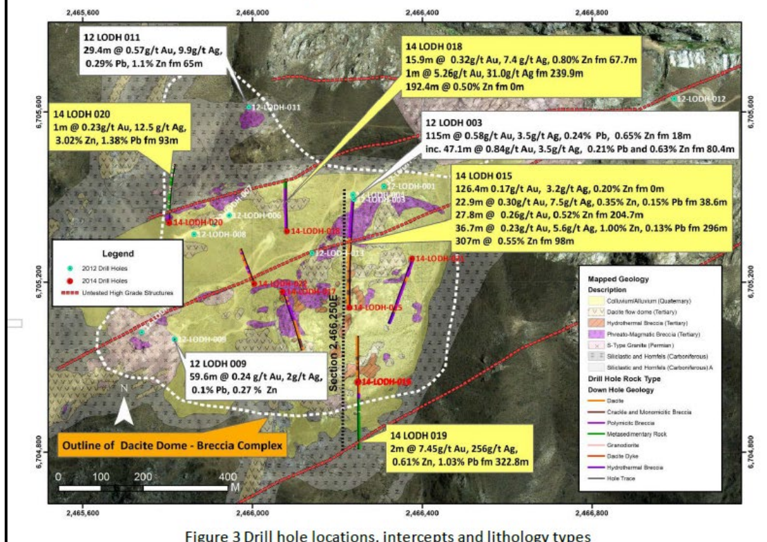
Figure 3 Drill hole locations, intercepts and lithology types
