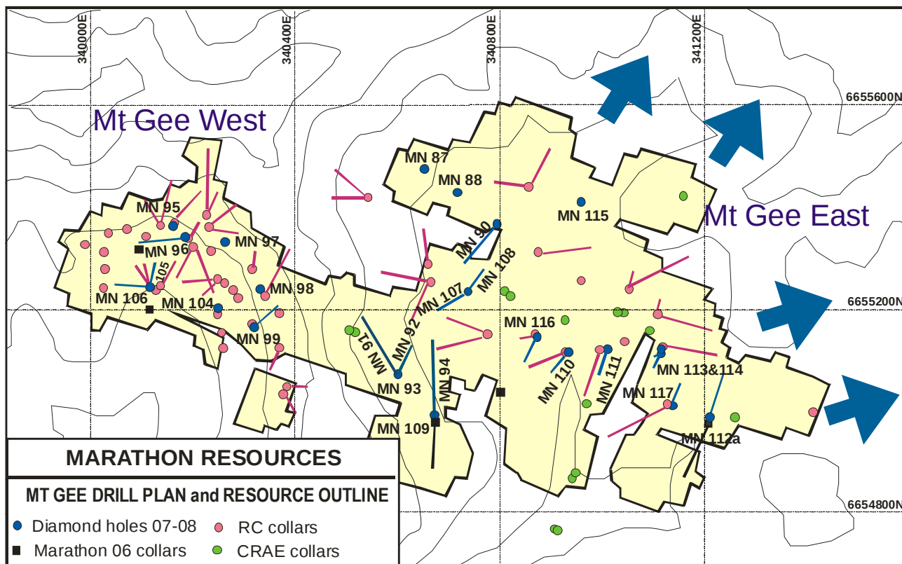
Figure 1 – Location of recent diamond holes with Mt Gee resource outline at 300ppm U_3O_8 cut-off. Note the open directions of mineralisation to the East and Northeast
