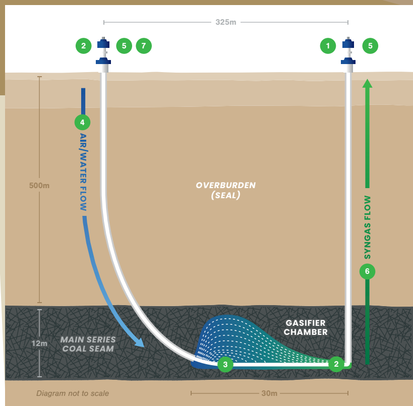
ISG process showing the below ground single ISG gasifier chamber.
