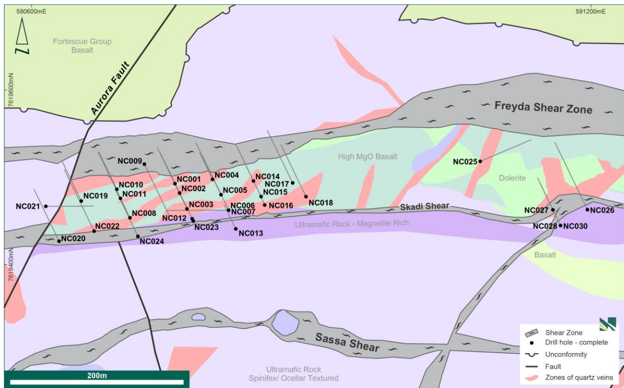
Figure 3: Nunyerry North geological interpretation and drill hole location plan.
