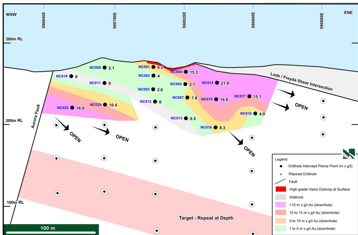
Figure 4: Nunyerry North long section (looking NNW) showing m x g/t Au (downhole width) for the Main Lode #1
