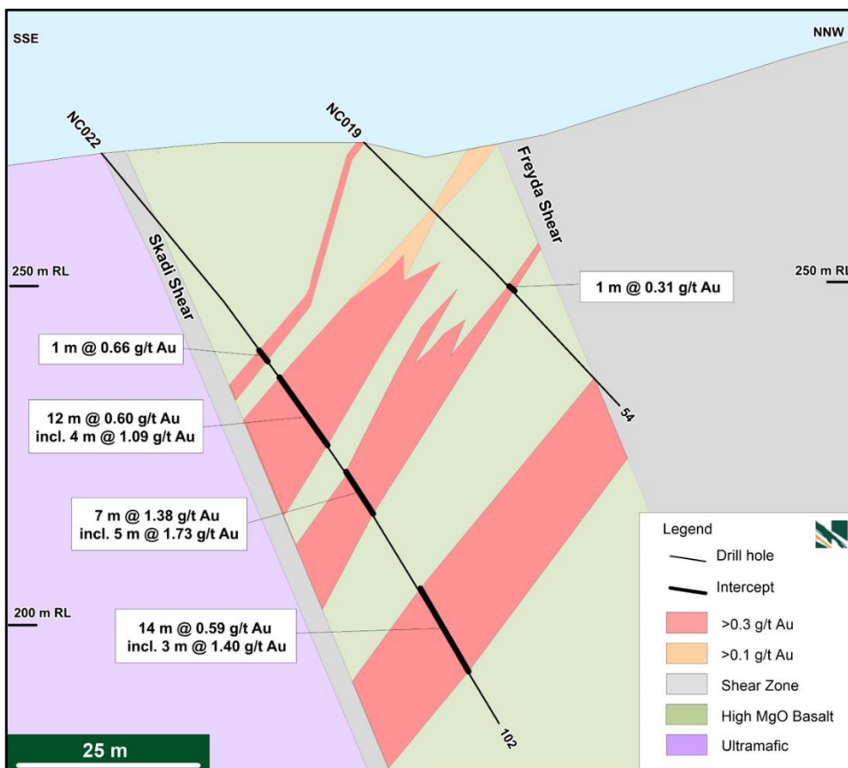
Figure 6: Nunyerry North cross section 590660E (looking WSW).
