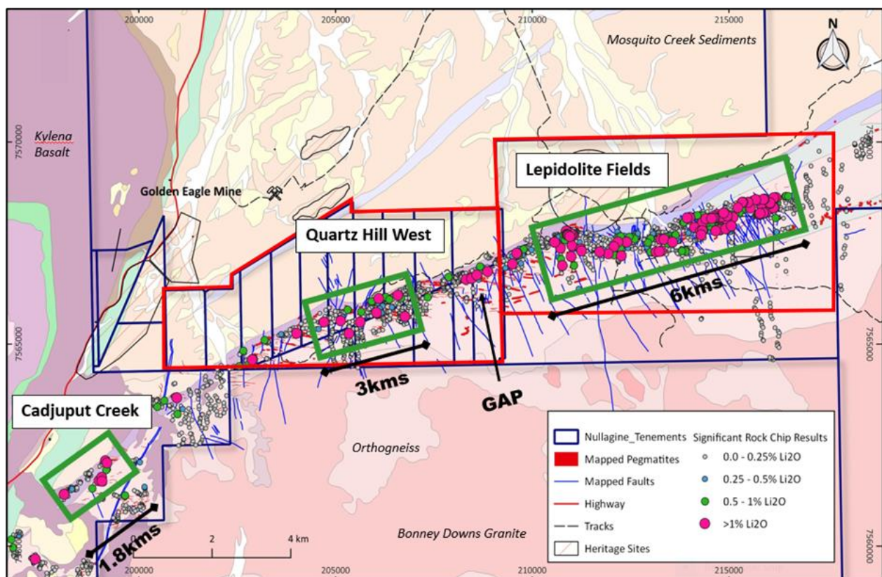
Figure 3: Lepidolite Fields and Quartz Hill West exploration areas identified through mapping and surface sampling.
