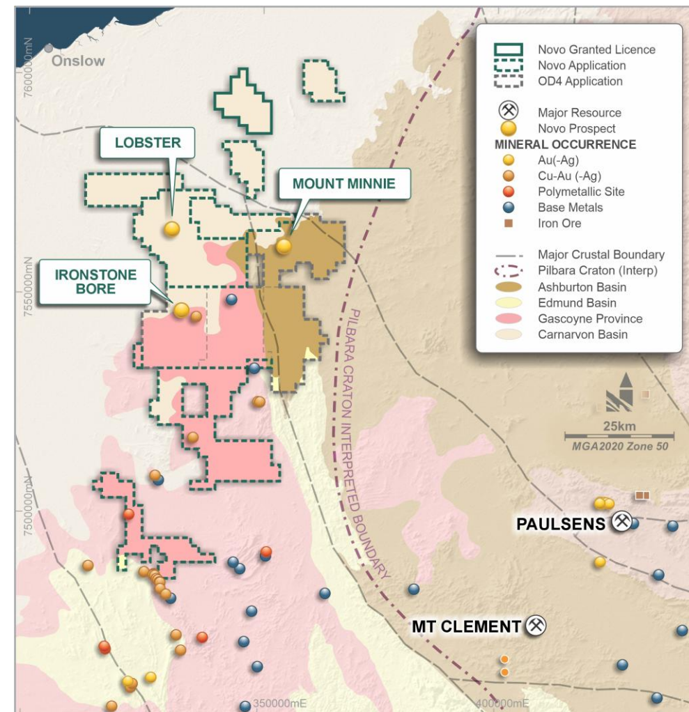
Toolunga Project in the Onslow District tenure and geological setting
