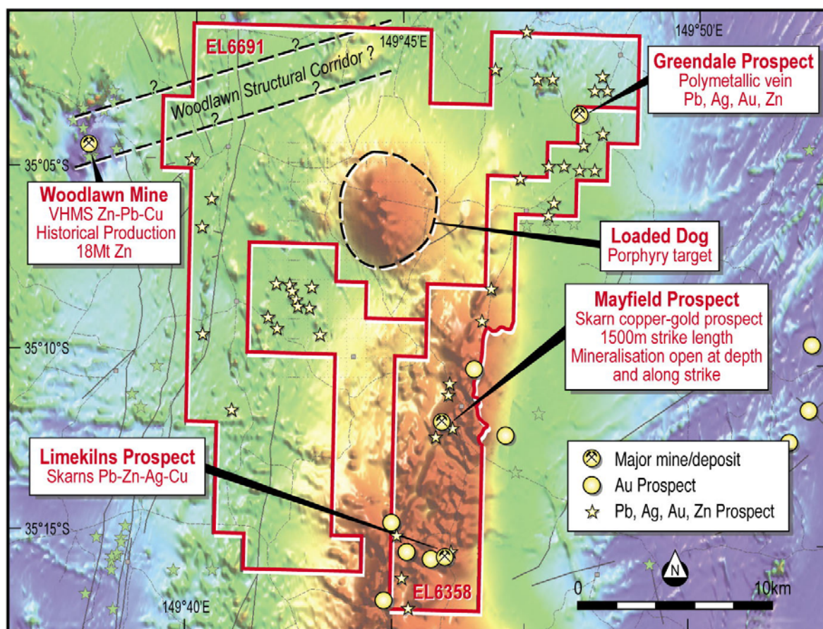
Figure 1: Monaro tenement outline over aeromagnetic image and showing the main exploration targets
