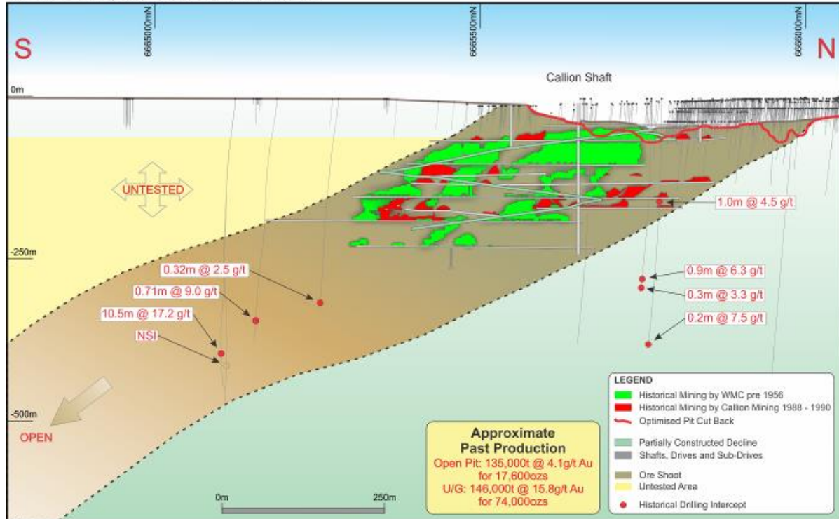
Figure 2. Long Section (looking west)
