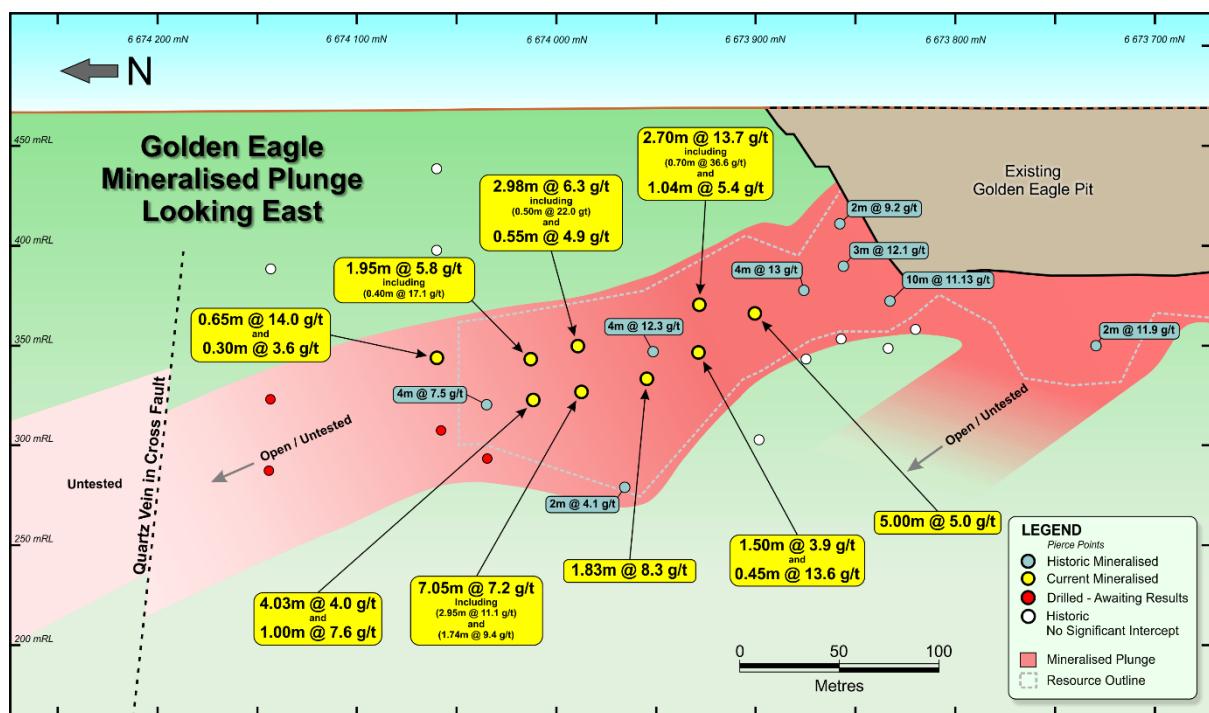
Figure 1 - Long Section looking east, March 2015 Resource model with Recent drill holes
