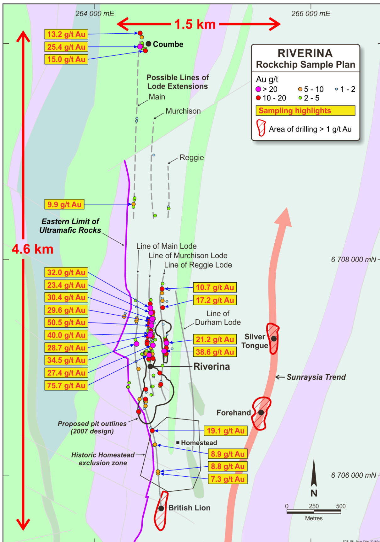
Figure 4: Riverina rock chip sampling location plan
