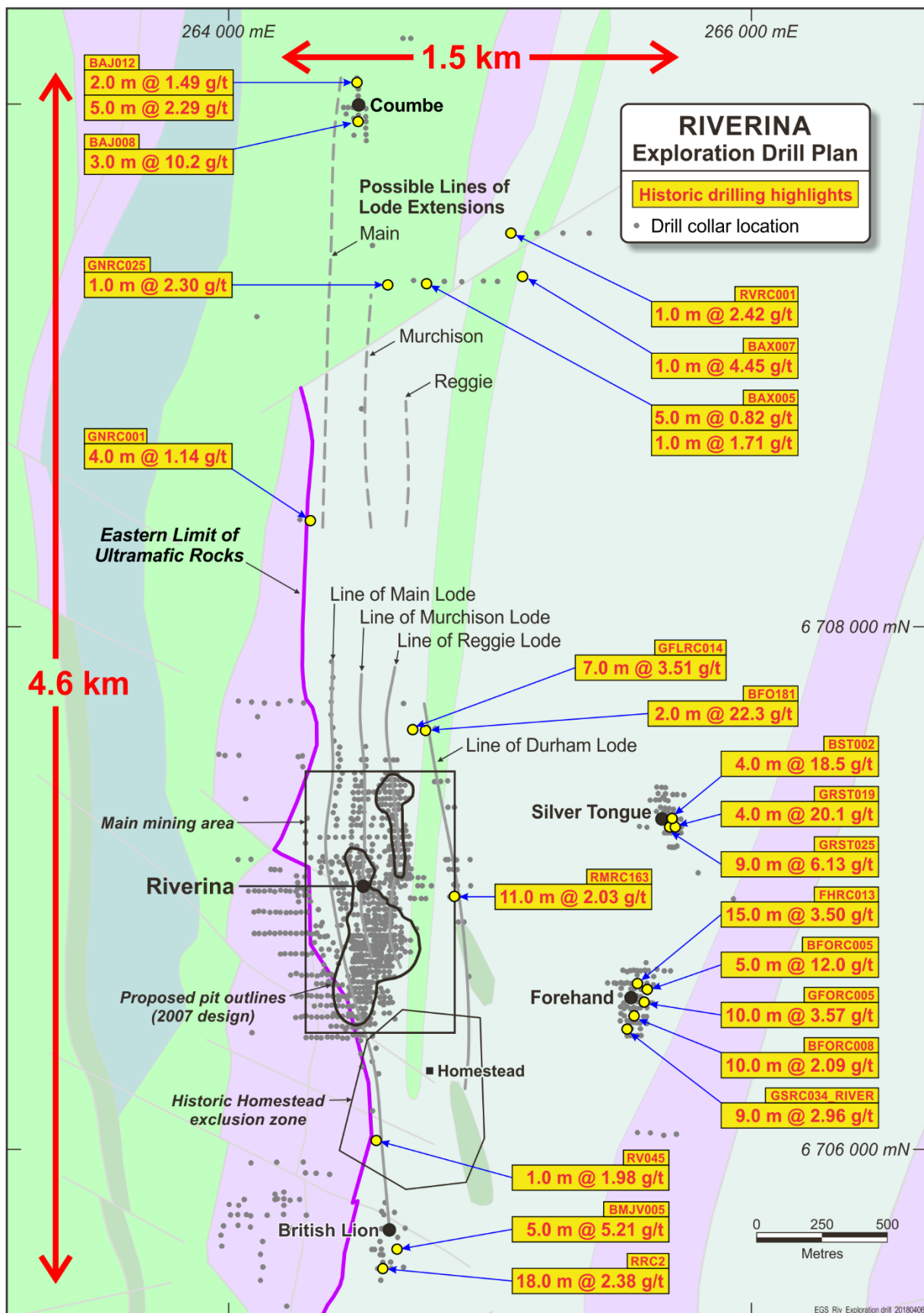
Figure 5: Riverina exploration drill plan with historic highlights shown.
