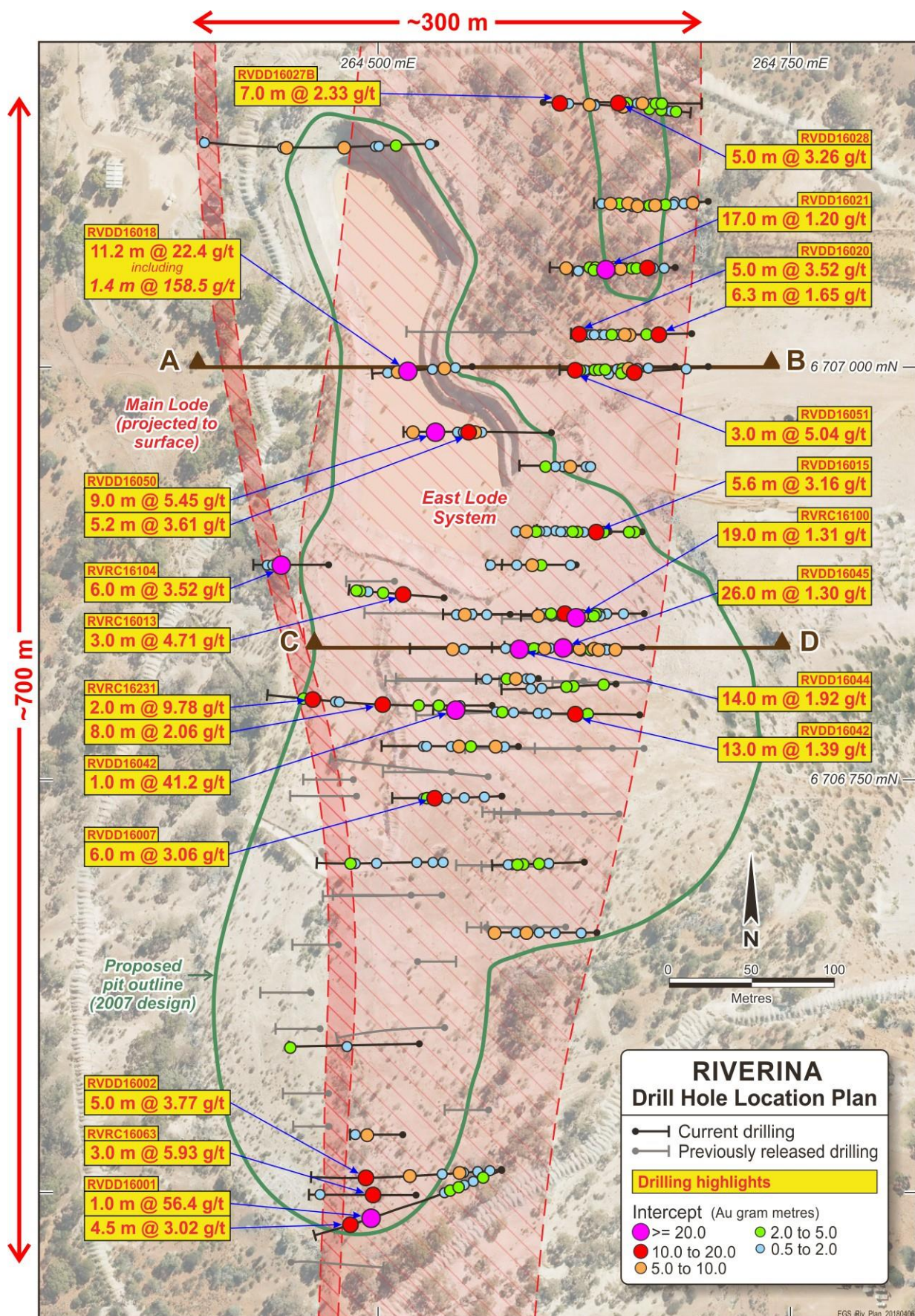
Figure 3: Riverina drill hole location plan covering the main mining area (also shown are section locations & Lode systems open to the north and south)
