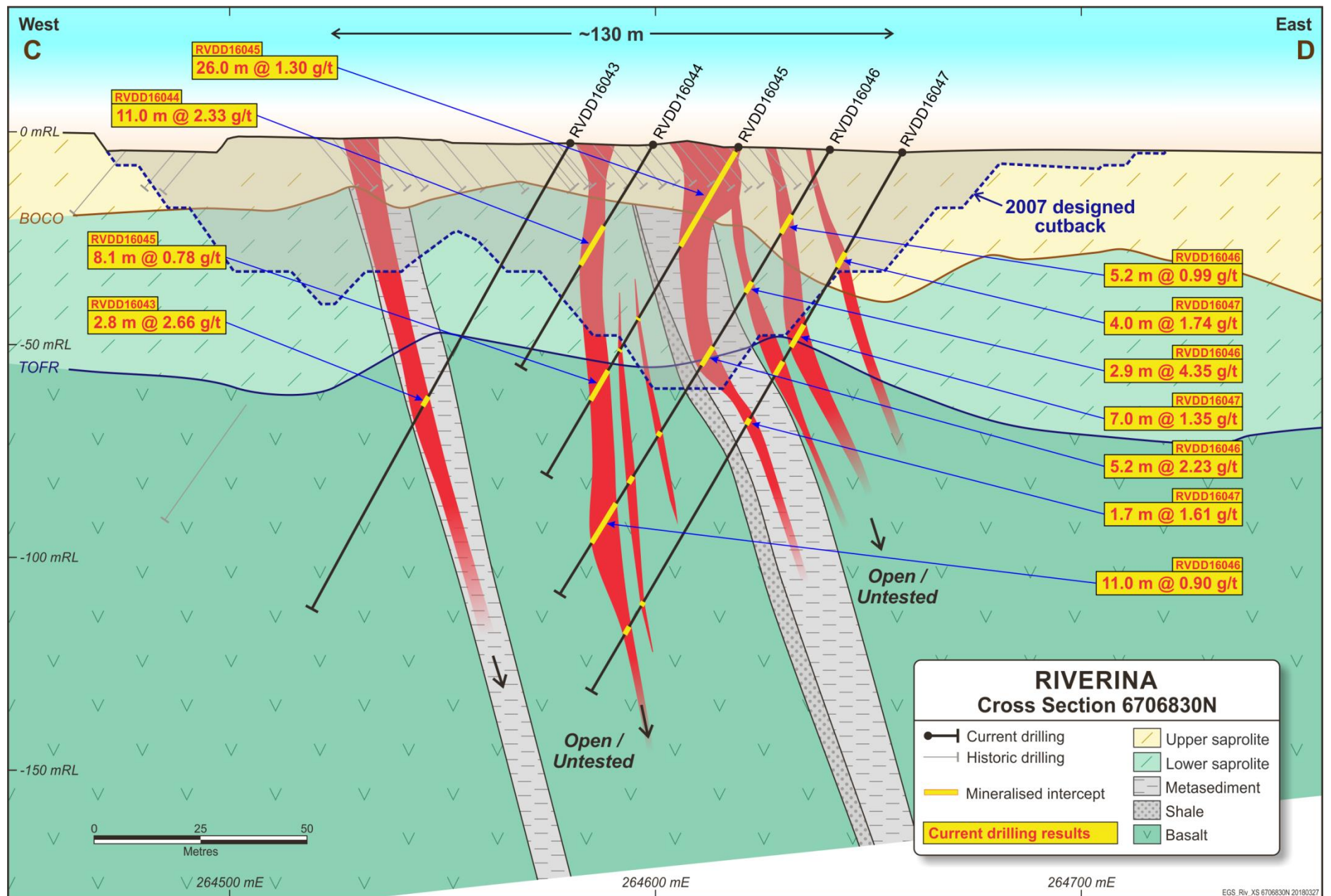
Figure 7: Cross Section 6706830N (East Lode System)
