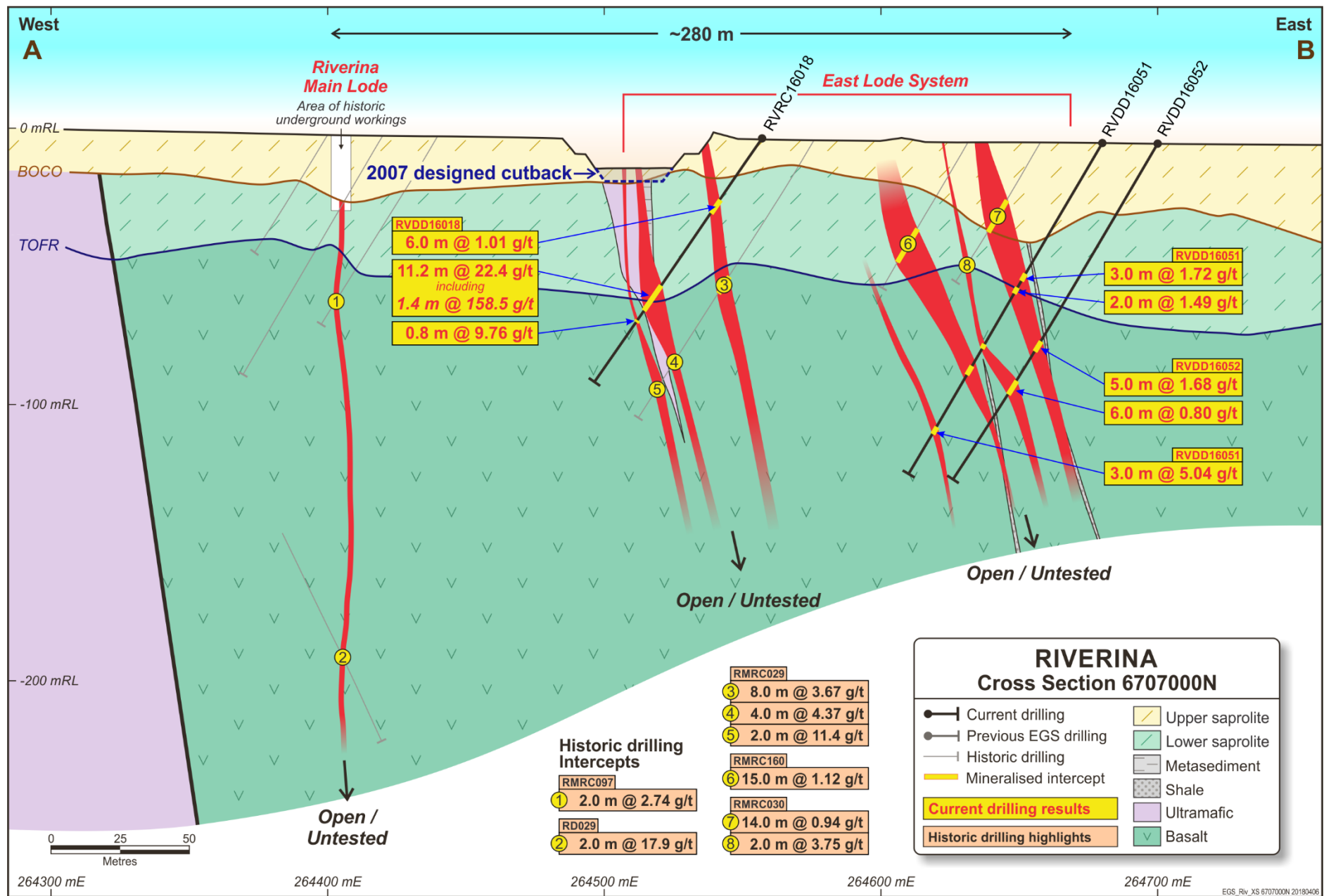
Figure 6: Cross Section 6707000N
