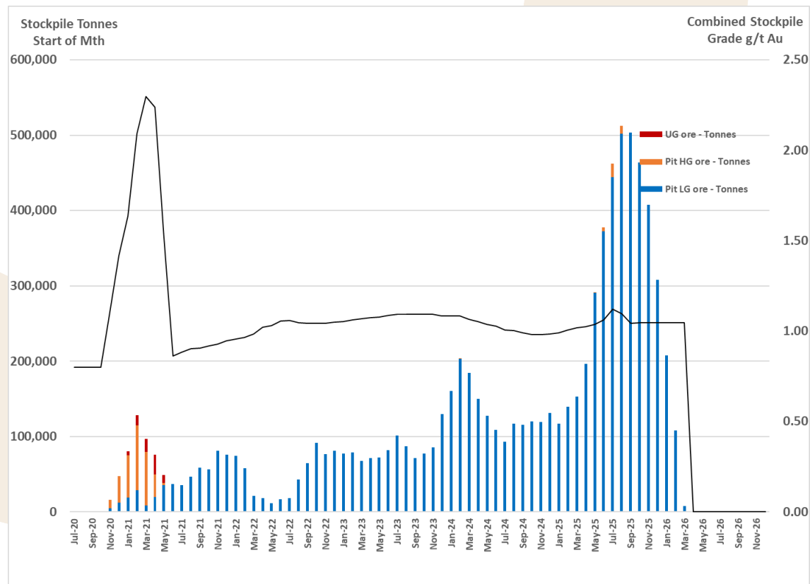
Figure 4.5: Stockpiling Schedule
